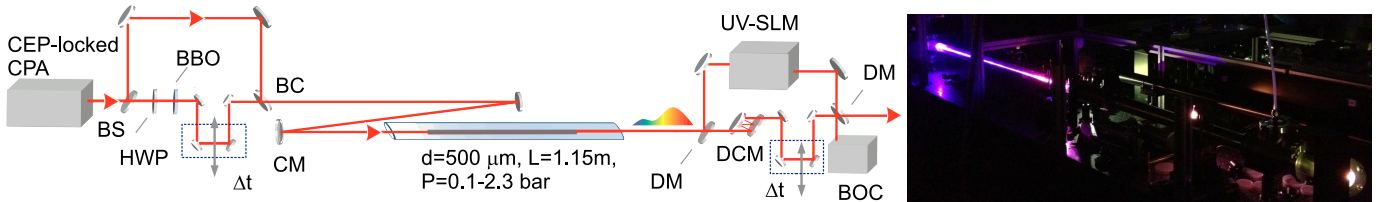
Fig. 13. (Left) Optical waveform synthesizer based on induced-phase modulation in a two-color-driven gas-filled hollow-core fiber compressor: BS, beam splitter; BBO, \beta -barium borate crystal; HWP, half-wave plate; BC, beam combiner; CM, concave mirror; DM, dichroic mirror; DCM, double-chirped mirror; UV-SLM, UV spatial light modulator; BOC, balanced optical cross-correlator. (Right) Photo of the experiment. The red and blue input pulses are visible on the left, the white-light supercontinuum can be seen (partly obstructed) on the right.
