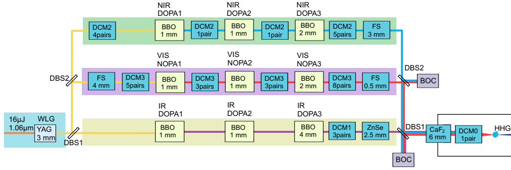
Fig. 7. Map of the dispersion management: WL, white-light generation; DBS, dichroic beam splitter; FS, fused silica; DCM, double-chirped mirror (number of pairs as indicated).
