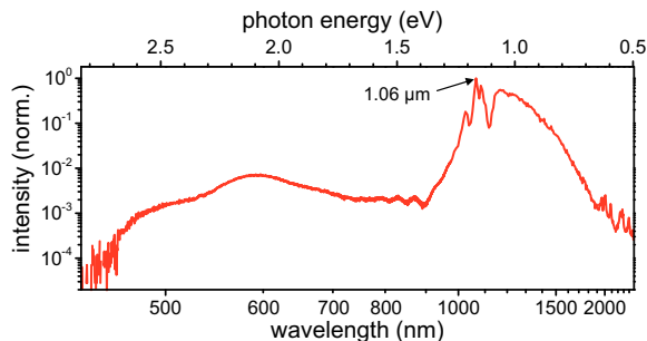
Fig. 2. Passively CEP-stabilized white-light seed continuum generated in a 3-mm-thick YAG crystal pumped by the second harmonic ( 1.06 \mu\text{m} ) of the CEP-stable idler [63] of the NIR OPA shown in Fig. 1.
