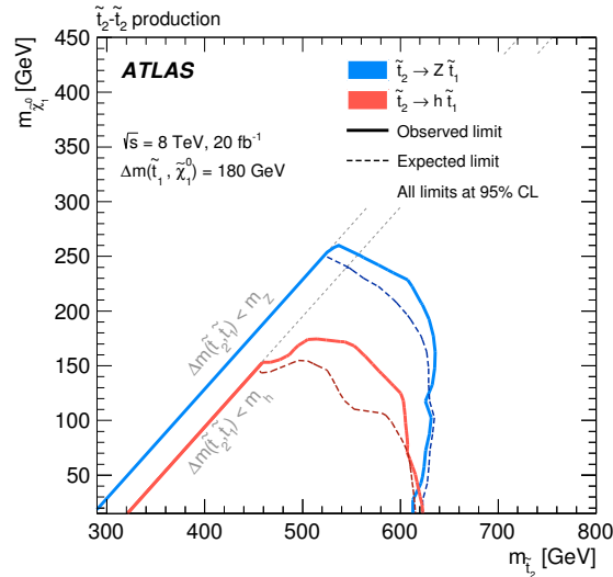
Figure 9: Exclusion limits at 95% CL in the scenario where \tilde{t}_2 pair production is assumed, followed by the decay \tilde{t}_2 \rightarrow Z\tilde{t}_1 (blue) or \tilde{t}_2 \rightarrow h\tilde{t}_1 (red) and then by \tilde{t}_1 \rightarrow t\tilde{\chi}_1^0 with a branching ratio of 100%, as a function of the \tilde{t}_2 and \tilde{\chi}_1^0 mass. The \tilde{t}_1 mass is determined by the relation m_{\tilde{t}_1} - m_{\tilde{\chi}_1^0} = 180 GeV. The dashed lines indicate the expected limit, the solid lines indicate the observed limit, and the dotted lines indicate the sensitivity to \pm 1\sigma variations of the signal theoretical uncertainties.
