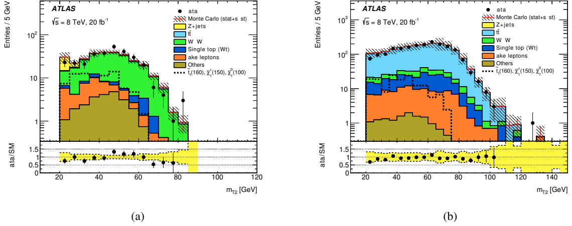
Figure 17: Distribution of the transverse mass m_{T2} in the (a) WW-VR2 and (b) WW-VRT regions defined in the text. The contributions from all SM processes are shown as a histogram stack. The component labelled as “Fake leptons” includes the estimate of the background from non-prompt leptons. The expected signal for a model of stop pair production with the stop decaying as \tilde{t}_1 \rightarrow b\tilde{\chi}_1^\pm \rightarrow b\ell^\pm\nu\tilde{\chi}_1^0 with m_{\tilde{t}_1} = 160 GeV, m_{\tilde{\chi}_1^\pm} = 150 GeV and m_{\tilde{\chi}_1^0} = 100 GeV is also shown. The lower panels show the ratio between the data and the SM prediction; the yellow band includes statistical and systematic uncertainties on the SM prediction.
