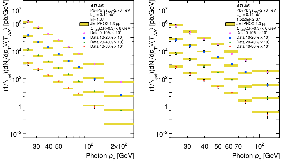
Figure 6: Fully corrected yields of prompt photons in four centrality intervals as a function of p_T in |\eta| < 1.37 (left) and 1.52 \leq |\eta| < 2.37 (right) using tight selection, isolation cone size \Delta R_{\text{iso}} = 0.3 and isolation transverse energy of less than 6 GeV. JETPHOX calculations, for proton-proton collisions and using the same isolation criterion, are shown by the yellow bands. Statistical uncertainties are shown by the error bars. Systematic uncertainties on the photon yields shown by braces, which are smaller than the markers for some points. The scale uncertainties due to \langle T_{AA} \rangle are tabulated for each bin in Table 1.
