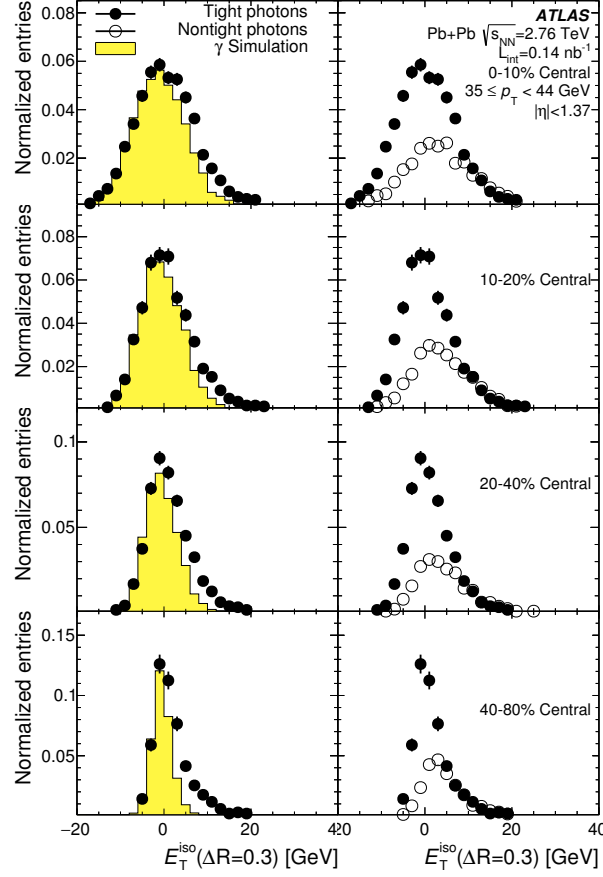
Figure 2: Distributions of photon isolation transverse energy in a \Delta R_{\text{iso}} = 0.3 cone for the four centrality bins in data (black points, normalized by the number of events and by the histogram bin width), for photons with 35 \leq p_T < 44.1 GeV. In the left column simulations (yellow histogram) are normalized to the data so that the integrals in the range E_T^{\text{iso}} < 0 are the same. The corresponding sample of nontight photon candidates, normalized to the distribution of tight photons for E_T^{\text{iso}} \geq 8 GeV is shown overlaid on the tight photon data in the right column to illustrate the source of the photons with large E_T^{\text{iso}} .
