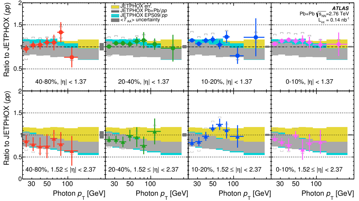
Figure 7: Fully corrected normalized yields of prompt photons as a function of p_T in |\eta| < 1.37 and 1.52 \leq |\eta| < 2.37 using tight photon selection, isolation cone size \Delta R_{\text{iso}} = 0.3 and isolation transverse energy of less than 6 GeV, divided by JETPHOX predictions for pp collisions, which implement the same isolation selection. The combined scale and PDF uncertainty on the JETPHOX calculation is shown by the yellow area. In addition two other JETPHOX calculations are shown, also divided by the pp results: Pb+Pb collisions with no nuclear modification (solid black line), and Pb+Pb collisions with EPS09 nuclear modifications (blue area). Statistical uncertainties are shown by the bars. Systematic uncertainties on the photon yields are combined and shown by the upper and lower braces. The scale uncertainties due only to \langle T_{AA} \rangle are tabulated for each bin in Table 1.
