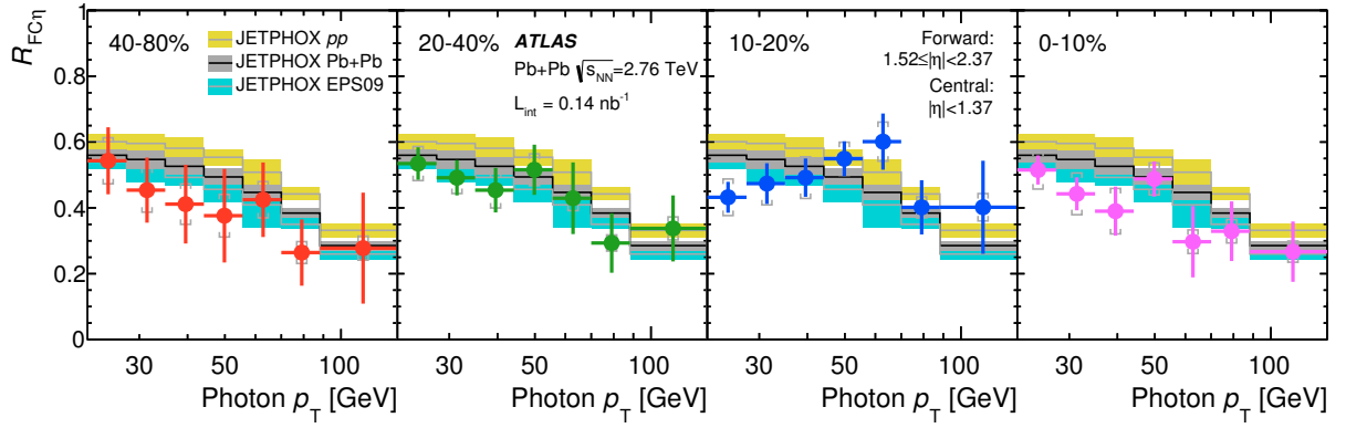
Figure 8: Fully corrected yields of prompt photons as a function of p_T in 1.52 \leq |\eta| < 2.37 divided by that measured in |\eta| < 1.37 using the tight photon selection, isolation cone size \Delta R_{\text{iso}} = 0.3 and isolation transverse energy of 6 GeV. The yield ratio is compared to JETPHOX 1.3 predictions that implement the same isolation selection, for three different configurations: for pp collisions (yellow area), Pb+Pb collisions with no nuclear modification (solid black line), and Pb+Pb collisions with EPS09 nuclear modifications (blue area). Statistical uncertainties are shown by the bars. Systematic uncertainties on the photon yields are combined and shown by the braces.
