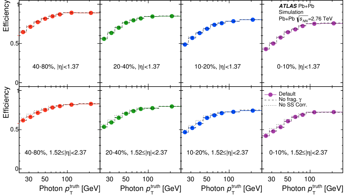
Figure 5: Total photon efficiency as a function of photon p_T and event centrality averaged over |\eta| < 1.37 (top row) and 1.52 \leq |\eta| < 2.37 (bottom row). Variations of the efficiency from removing the small corrections to the simulated shower-shape variable, and from removing fragmentation photons from the simulations are shown by dotted and dashed lines, respectively.
