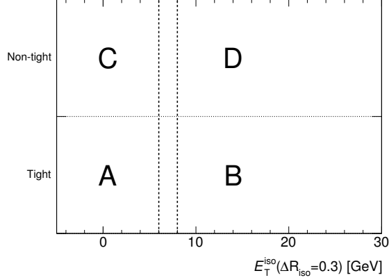
Figure 3: Illustration of the double sideband approach, showing the two axes for partitioning photon candidates: region A is the “signal region” (tight and isolated photons), region B contains tight, nonisolated photons, region C contains nontight isolated photons, and region D contains nontight and nonisolated photons.
