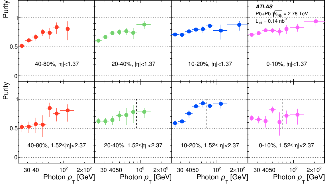
Figure 4: Photon purity as a function of collision centrality (left to right) and photon p_T , for photons measured in |\eta| < 1.37 (top row) and 1.52 \leq |\eta| < 2.37 (bottom row). The p_T intervals to the right of the vertical dotted line indicated in some bins use the extrapolation method described in the text to account for low event counts in the sidebands.
