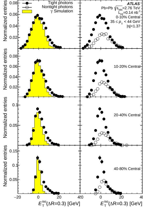
Figure 2: Distributions of photon isolation transverse energy in a \Delta R_{\text{iso}} = 0.3 cone for the four centrality bins in data (black points, normalized by the number of events and by the histogram bin width), for photons with 35 \leq p_T < 44.1 GeV. In the left column simulations (yellow histogram) are normalized to the data so that the integrals in the range E_T^{\text{iso}} < 0 are the same. The corresponding sample of nontight photon candidates, normalized to the distribution of tight photons for E_T^{\text{iso}} \geq 8 GeV is shown overlaid on the tight photon data in the right column to illustrate the source of the photons with large E_T^{\text{iso}} .
