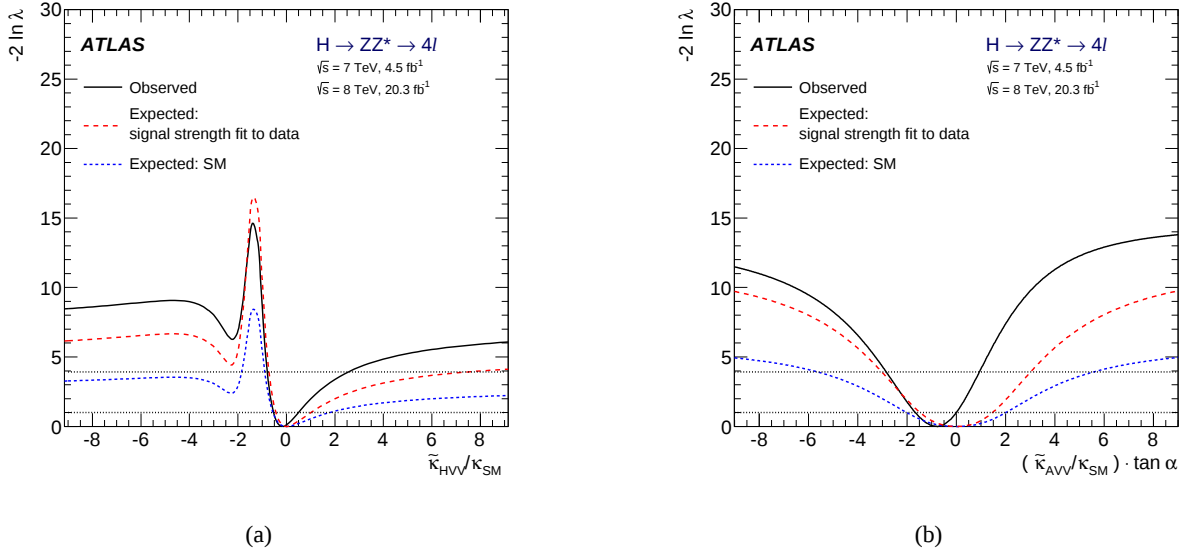
Figure 9: Expected and observed distributions of the test statistic for fits of (a) \tilde{\kappa}_{HVV}/\kappa_{SM} and (b) (\tilde{\kappa}_{AVV}/\kappa_{SM}) \cdot \tan \alpha for the H \rightarrow ZZ^* \rightarrow 4\ell analysis. The expected curves are calculated assuming the SM J^P = 0^+ signal and produced with the SM signal strength \mu = 1 and with the signal strengths fitted to data. The horizontal dotted black lines represent the levels of -2 \ln \lambda above which the values of coupling ratios under study are excluded above 68% and 95% CL, respectively.
