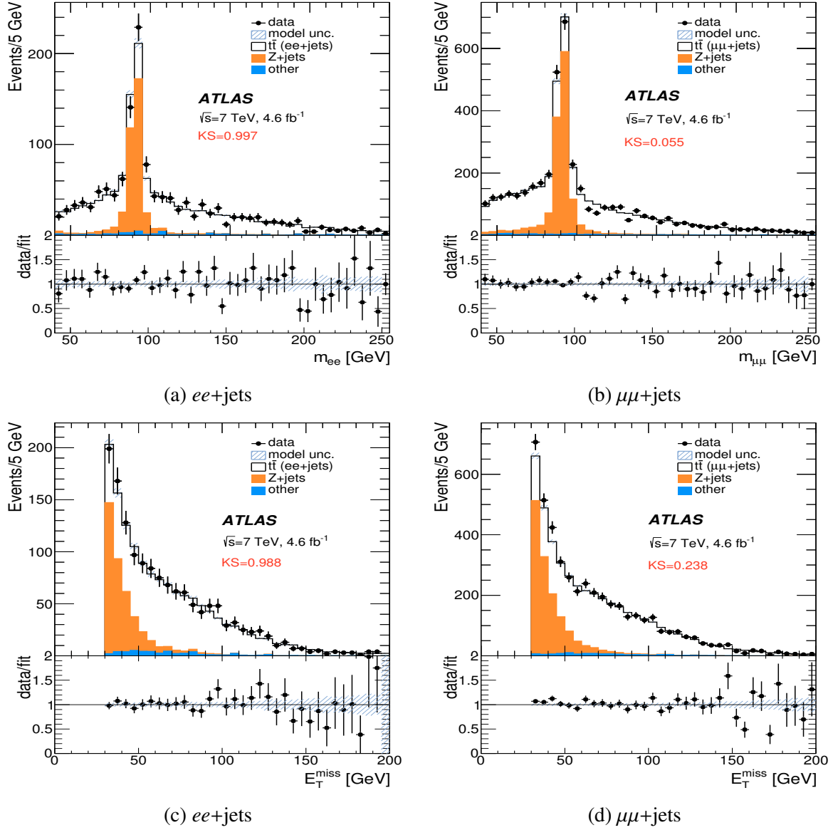
Figure 6: Dilepton invariant masses (a) m_{ee} , (b) m_{\mu\mu} , and E_T^{\text{miss}} distributions for events with two isolated leptons, E_T^{\text{miss}} > 30 GeV, at least two jets, and at least one b -tag in the (c) ee+jets and (d) \mu\mu+jets channels. The Z+jet entries include a small contribution from Z \rightarrow \tau^+ \tau^- with both \tau leptons decaying to e or \mu . The ratio plots show the result of dividing the data points by the fit. The model uncertainty (model unc.) is the sum in quadrature of the statistical uncertainties of the templates used in the fits. KS is the value of the Kolmogorov-Smirnov goodness-of-fit test.
