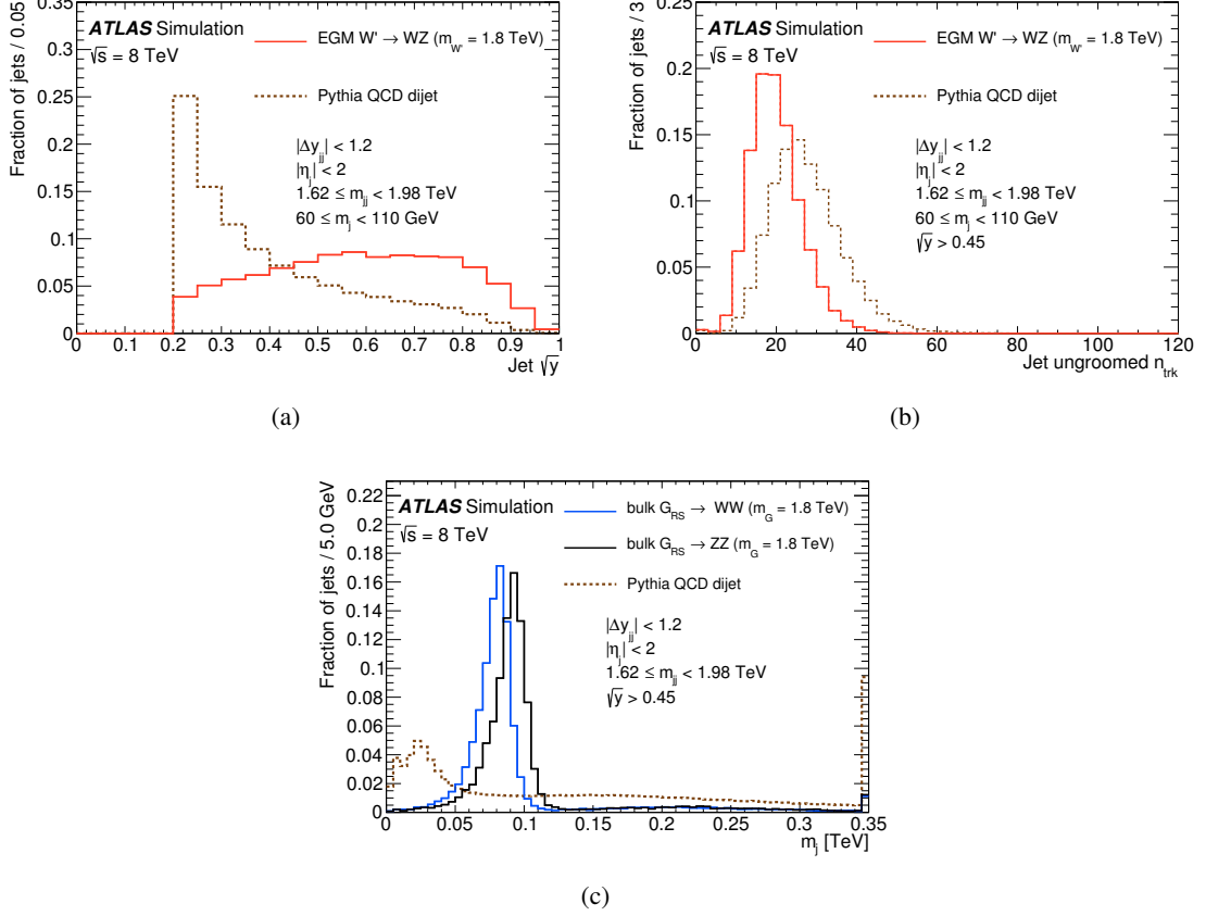
Figure 1: The distribution of the boson-tagging variables (a) subjet momentum balance \sqrt{y} , (b) number of tracks n_{\text{trk}} matched to the jet, and (c) mass m_j of the groomed jet, in simulated signal and background events. The signal and background distributions are normalised to unit area, and the last bin of each histogram includes the fraction of events falling outside of the displayed range. Requirements are placed on the events used to ensure that the kinematics of the signal and background events are comparable.
