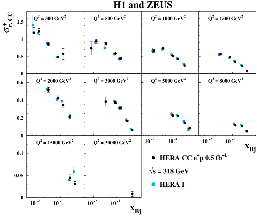
Figure 13: The combined HERA data for the inclusive CC e^+p reduced cross sections as a function of x_{Bj} for the 10 different values of Q^2 compared to the results from HERA I alone [2]. The individual measurements are displaced horizontally for better visibility. Error bars represent the total uncertainties.
