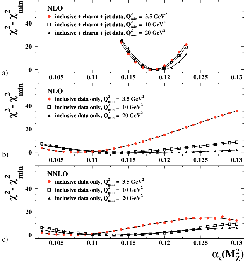
Figure 65: \Delta\chi^2 = \chi^2 - \chi^2_{\min} vs. \alpha_s(M_Z^2) for pQCD fits with different Q_{\min}^2 using data on (a) inclusive, charm and jet production at NLO, (b) inclusive ep scattering only at NLO and (c) inclusive ep scattering only at NNLO.
