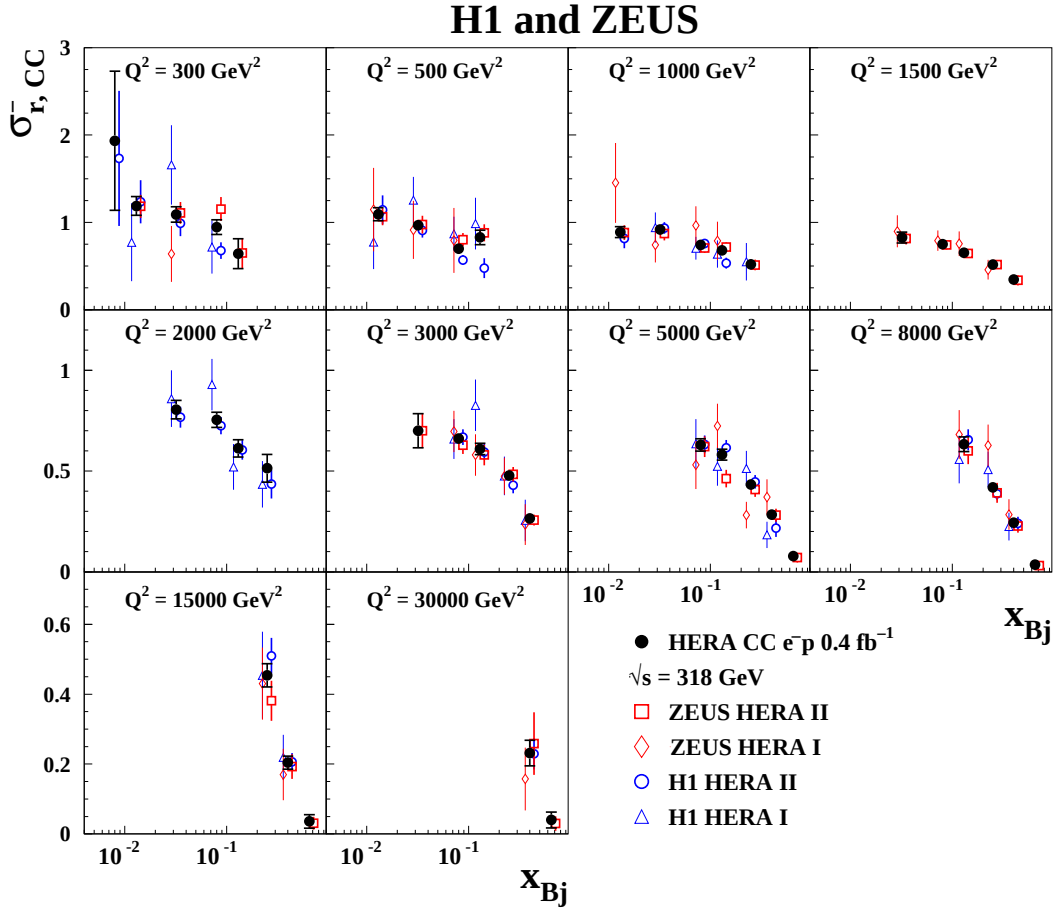
Figure 14: The combined HERA data for the inclusive CC e^-p reduced cross sections as a function of x_{Bj} for the 10 different values of Q^2 compared to the individual H1 and ZEUS data. The individual measurements are displaced horizontally for better visibility. Error bars represent the total uncertainties.
