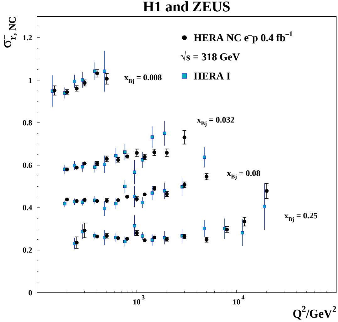
Figure 7: The combined HERA data for the inclusive NC e^-p reduced cross section as a function of Q^2 for four selected values of x_{Bj} compared to the results from HERA I alone [2]. The two measurements are displaced horizontally for better visibility. Error bars represent the total uncertainties.
