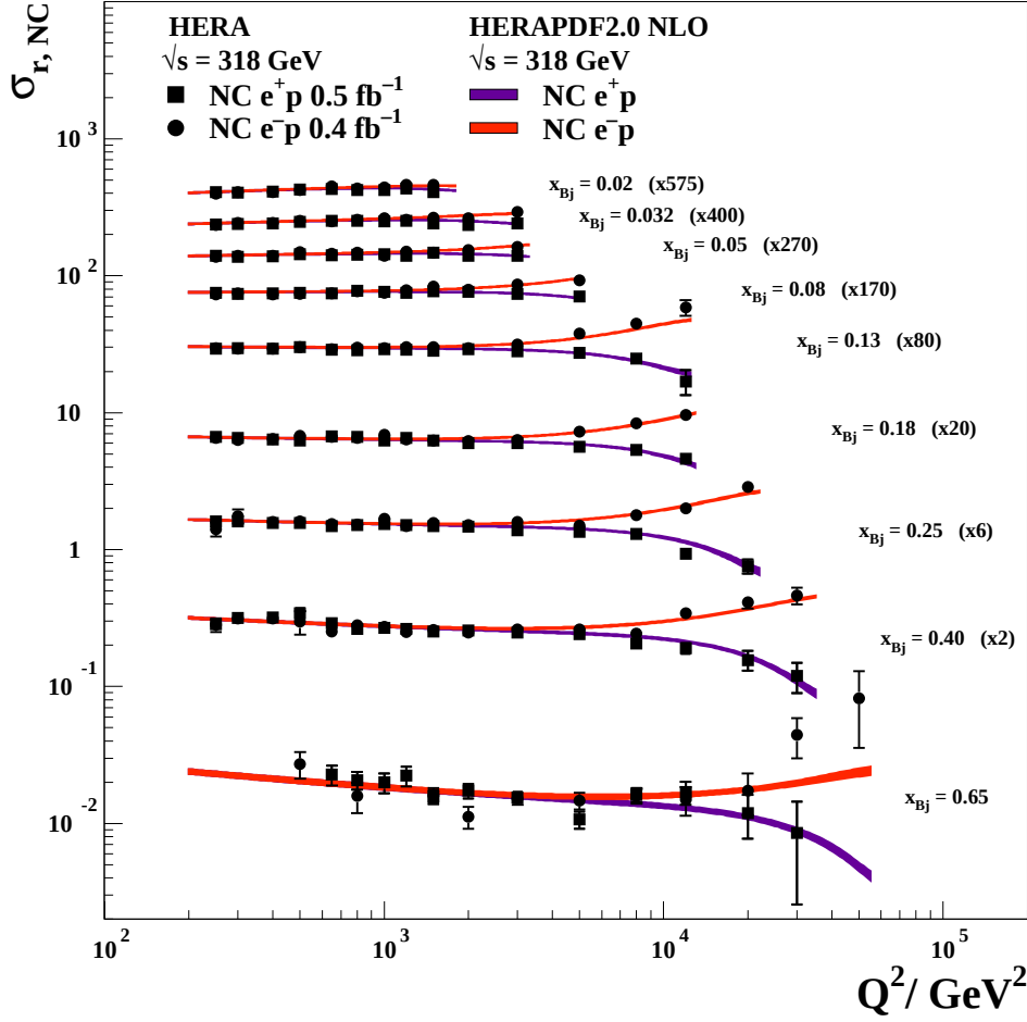
Figure 75: The combined HERA data for the inclusive NC e^+ p and e^- p reduced cross sections as a function of Q^2 for selected values of x_{Bj} at \sqrt{s} = 318 \text{ GeV} with overlaid predictions of HERAPDF2.0 NLO. The bands represent the total uncertainties of the predictions.
