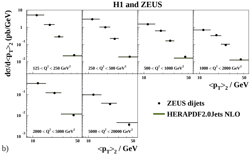
Figure 70: a) Differential jet cross-sections, d\sigma/dp_T , in bins of Q^2 between 125 and 20000 \text{GeV}^2 as measured by ZEUS. b) Differential dijet cross-sections, d\sigma/d\langle p_T \rangle_2 , in bins of Q^2 between 125 and 20000 \text{GeV}^2 as measured by ZEUS. The variable \langle p_T \rangle_2 denotes the average p_T of the two jets. Also shown are predictions from HERAPDF2.0Jets. The bands represent the total uncertainty on the predictions excluding scale uncertainties.
