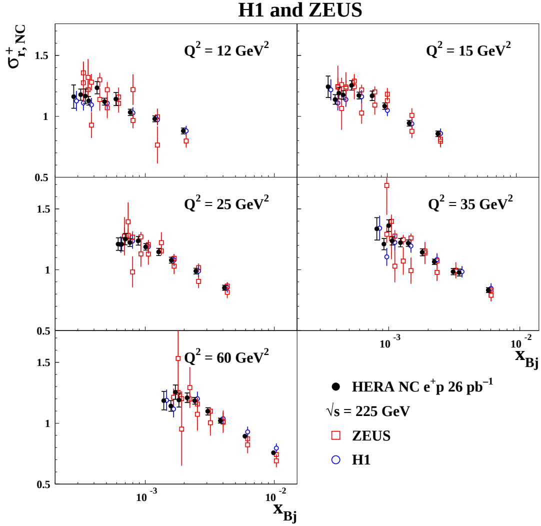
Figure 9: The combined HERA data for the inclusive NC e^+p reduced cross sections at \sqrt{s} = 225 GeV as a function of x_{Bj} for five selected values of Q^2 compared to the individual H1 and ZEUS data. The individual measurements are displaced horizontally for better visibility. The ZEUS points at the same x_{Bj} and Q^2 values are from two different data sets. Error bars represent the total uncertainties.
