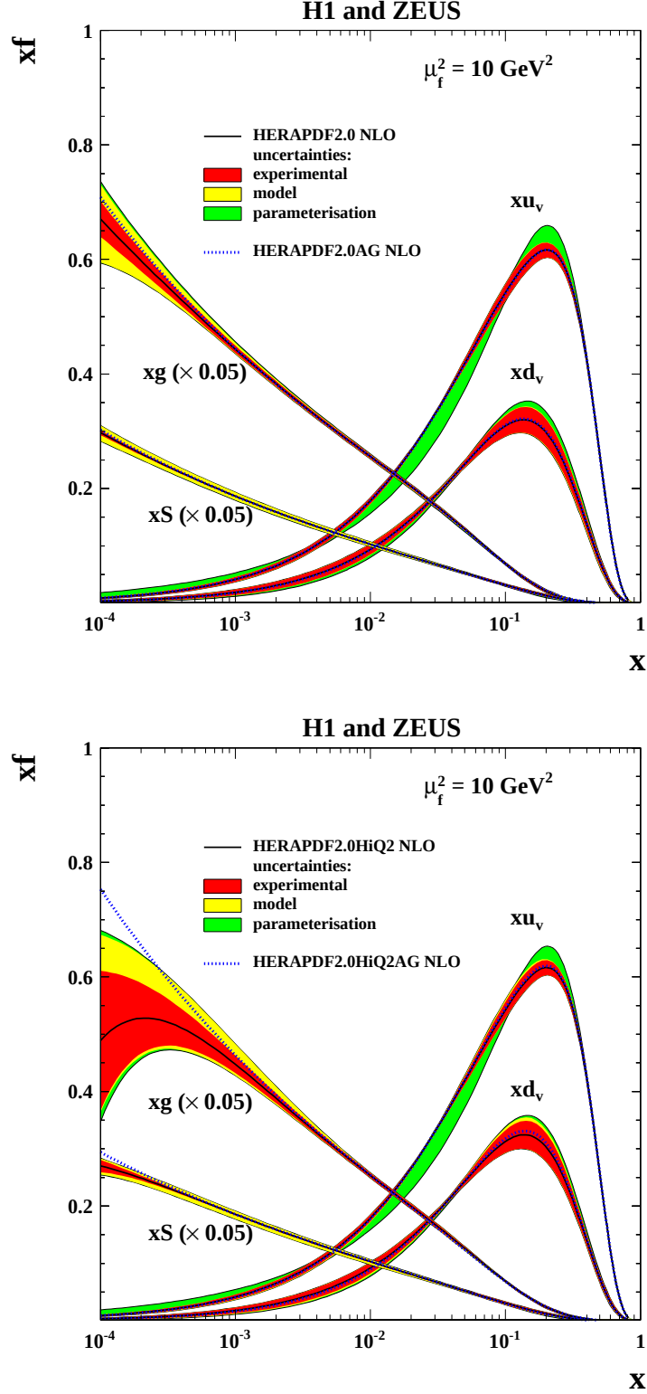
Figure 52: The parton distribution functions xu_v , xd_v , xS = 2x(\bar{U} + \bar{D}) and xg of HERAPDF2.0 NLO at \mu_f^2 = 10 \text{ GeV}^2 with Q_{\min}^2 = 3.5 \text{ GeV}^2 (top) and of HERAPDF2.0HiQ2 with Q_{\min}^2 = 10 \text{ GeV}^2 (bottom). The gluon and sea distributions are scaled down by a factor of 20. The experimental, model and parameterisation uncertainties are shown. The dotted lines represent HERAPDF2.0AG and HERAPDF2.0AG HiQ2.
