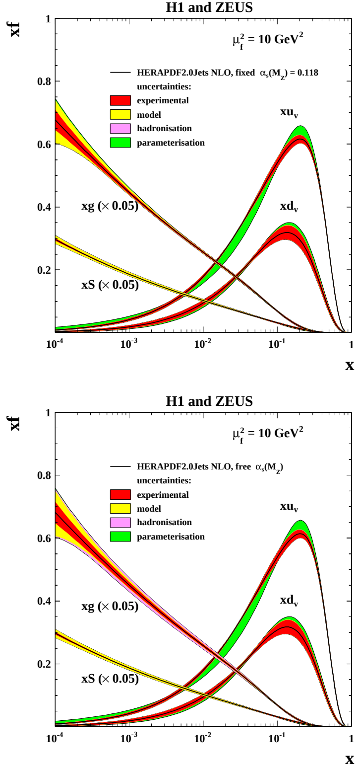
Figure 66: The parton distribution functions xu_v , xd_v , xS = 2x(\bar{U} + \bar{D}) and xg of HERAPDF2.0Jets NLO at \mu_f^2 = 10 \text{ GeV}^2 with fixed \alpha_s(M_Z^2) = 0.118 (top) and free \alpha_s(M_Z^2) (bottom). The experimental, model and parameterisation uncertainties are shown. The hadronisation uncertainty is also included, but it is only visible for the fit with free \alpha_s(M_Z^2) .
