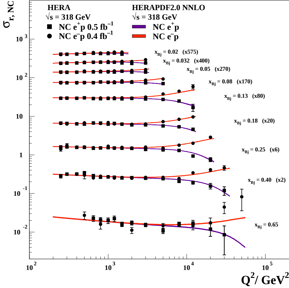
Figure 76: The combined HERA data for the inclusive NC e^+ p and e^- p reduced cross sections as a function of Q^2 for selected values of x_{Bj} at \sqrt{s} = 318 \text{ GeV} with overlaid predictions of HERAPDF2.0 NNLO. The bands represent the total uncertainties of the predictions.
