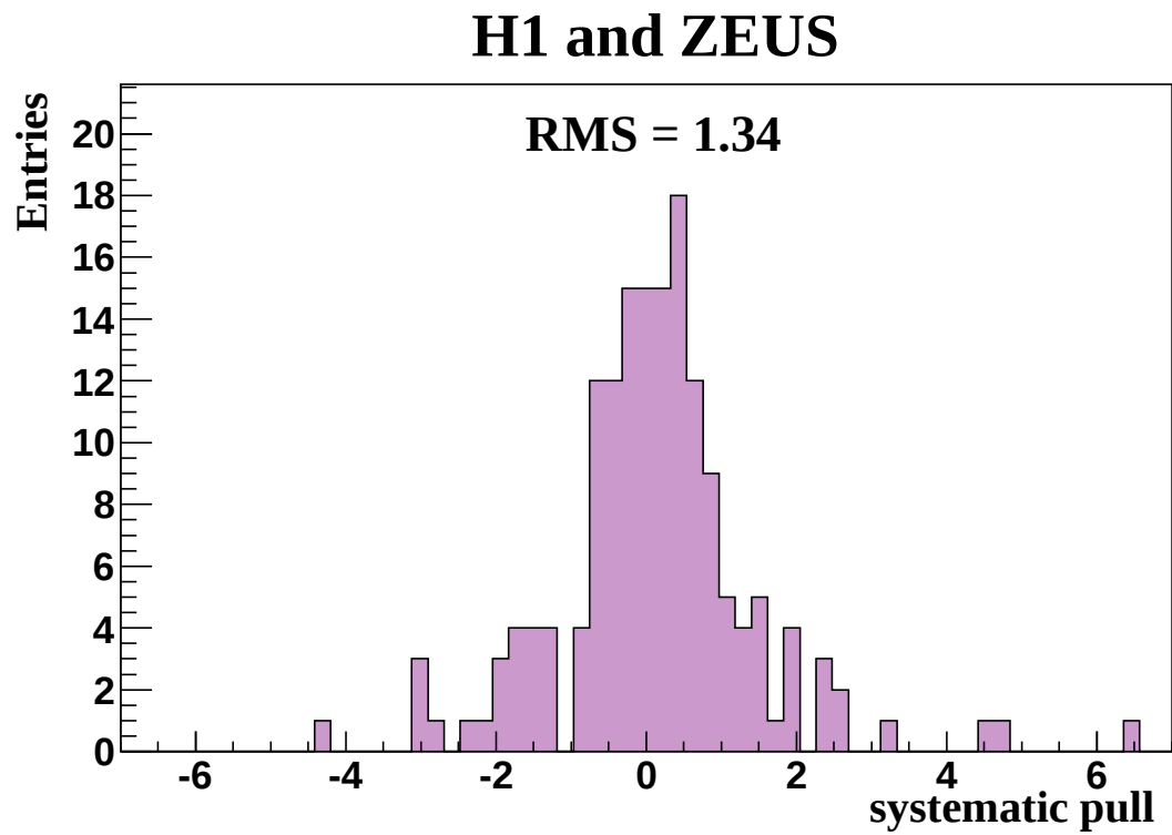
Figure 3: Distribution of pulls p_j for the correlated systematic uncertainties including global normalisations. There are no entries outside the histogram range. The root mean square, RMS, of the distribution is given.
