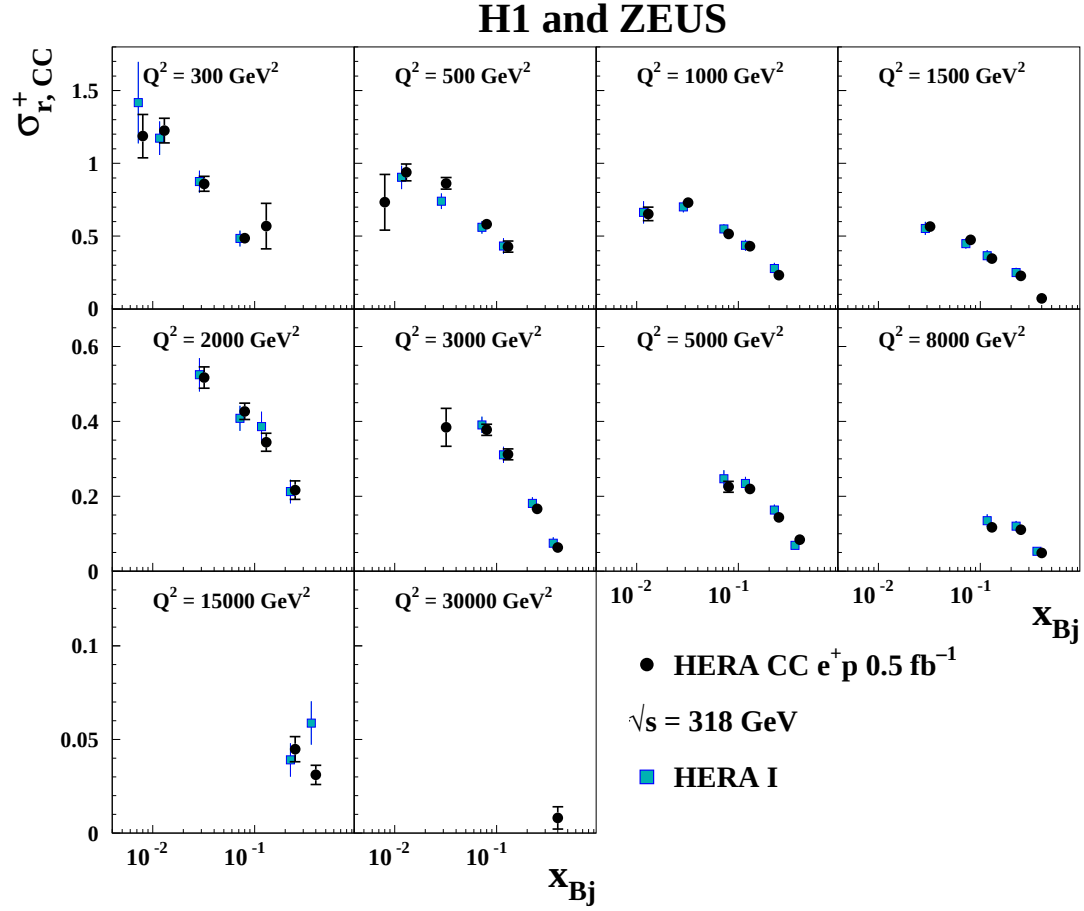
Figure 13: The combined HERA data for the inclusive CC e^+ p reduced cross sections as a function of x_{Bj} for the 10 different values of Q^2 compared to the results from HERA I alone [2]. The individual measurements are displaced horizontally for better visibility. Error bars represent the total uncertainties.
