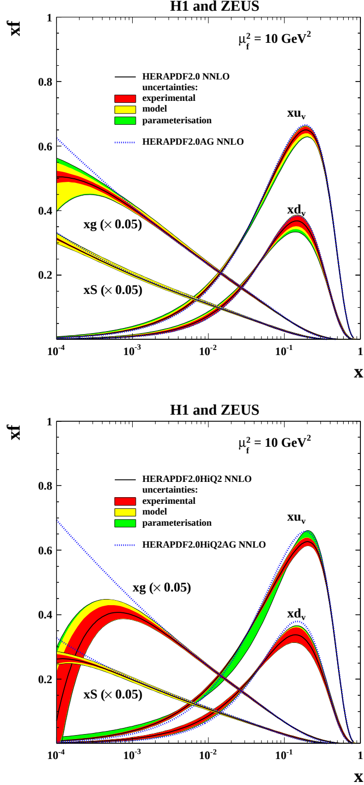
Figure 53: The parton distribution functions xu_v , xd_v , xS = 2x(\bar{U} + \bar{D}) and xg of HERAPDF2.0 NNLO at \mu_f^2 = 10 \text{ GeV}^2 with Q_{\min}^2 = 3.5 \text{ GeV}^2 (top) and of HERAPDF2.0HiQ2 with Q_{\min}^2 = 10 \text{ GeV}^2 (bottom). The gluon and sea distributions are scaled down by a factor 20. The experimental, model and parameterisation uncertainties are shown. The dotted lines represent HERAPDF2.0AG and HERAPDF2.0AG HiQ2.
