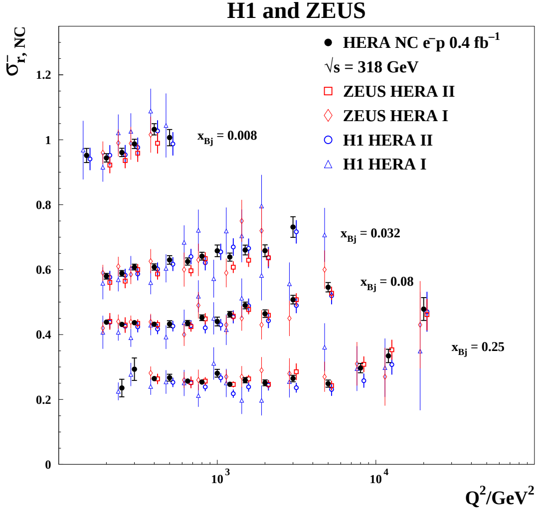
Figure 6: The combined HERA data for the inclusive NC e^-p reduced cross sections as a function of Q^2 for four selected values of x_{Bj} compared to the individual H1 and ZEUS data. The individual measurements are displaced horizontally for better visibility. Error bars represent the total uncertainties.
