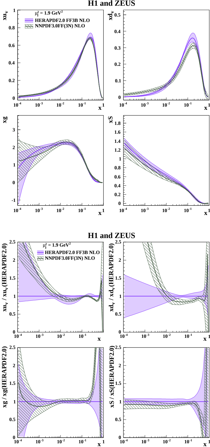
Figure 64: The parton distribution functions xu_v , xd_v , xg and xS = 2x(\bar{U} + \bar{D}) of HERAPDF2.0FF3B at the starting scale \mu_{f_0}^2 = 1.9 \text{ GeV}^2 compared to those of NNPDF3.0FF(3N). The top panel shows the distributions. The bottom panel shows the PDFs normalised to HERAPDF2.0FF3B. The uncertainties are given as differently hatched bands in both panels.
