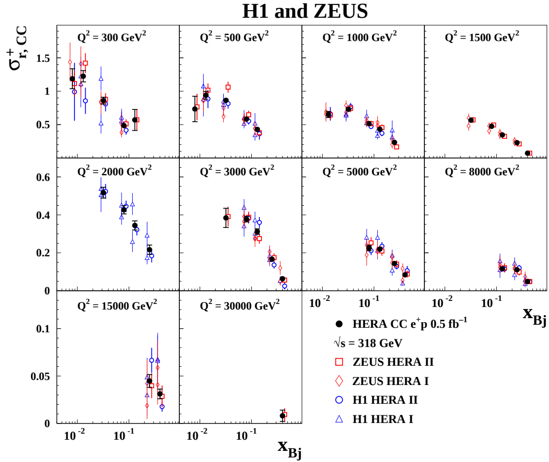
Figure 12: The combined HERA data for the inclusive CC e^+p reduced cross sections as a function of x_{Bj} for the 10 different values of Q^2 compared to the individual H1 and ZEUS data. The individual measurements are displaced horizontally for better visibility. Error bars represent the total uncertainties.
