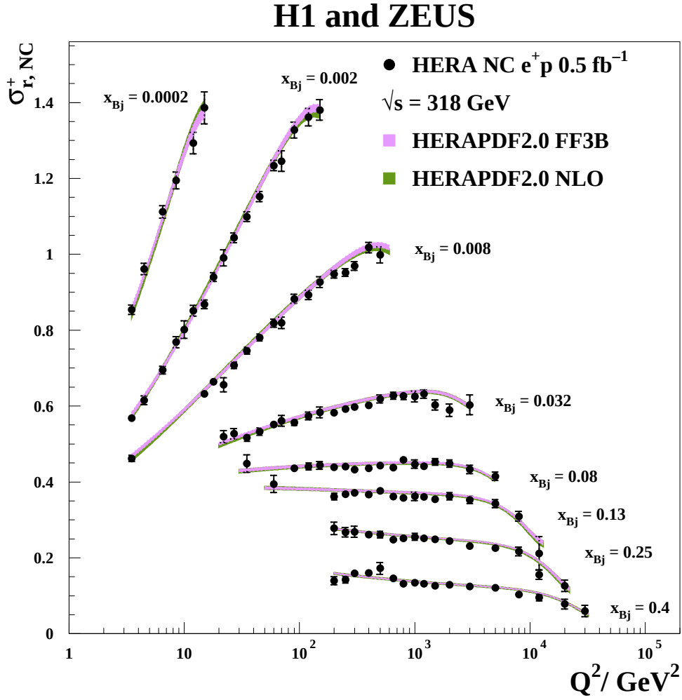
Figure 62: Selected combined HERA inclusive NC e^+p reduced cross sections compared to predictions of HERAPDF2.0 NLO and HERAPDF2.0FF3B. The two differently shaded bands represent the total uncertainties on the two predictions.
