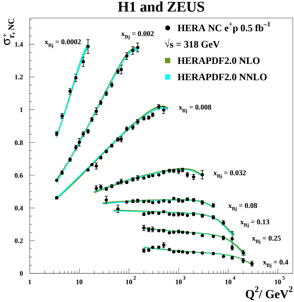
Figure 30: The combined high- Q^2 HERA inclusive NC e^+p reduced cross sections as partially shown already in Fig. 5 with overlaid predictions of HERAPDF2.0 NLO and NNLO. The two differently shaded bands represent the total uncertainties on the two predictions.
