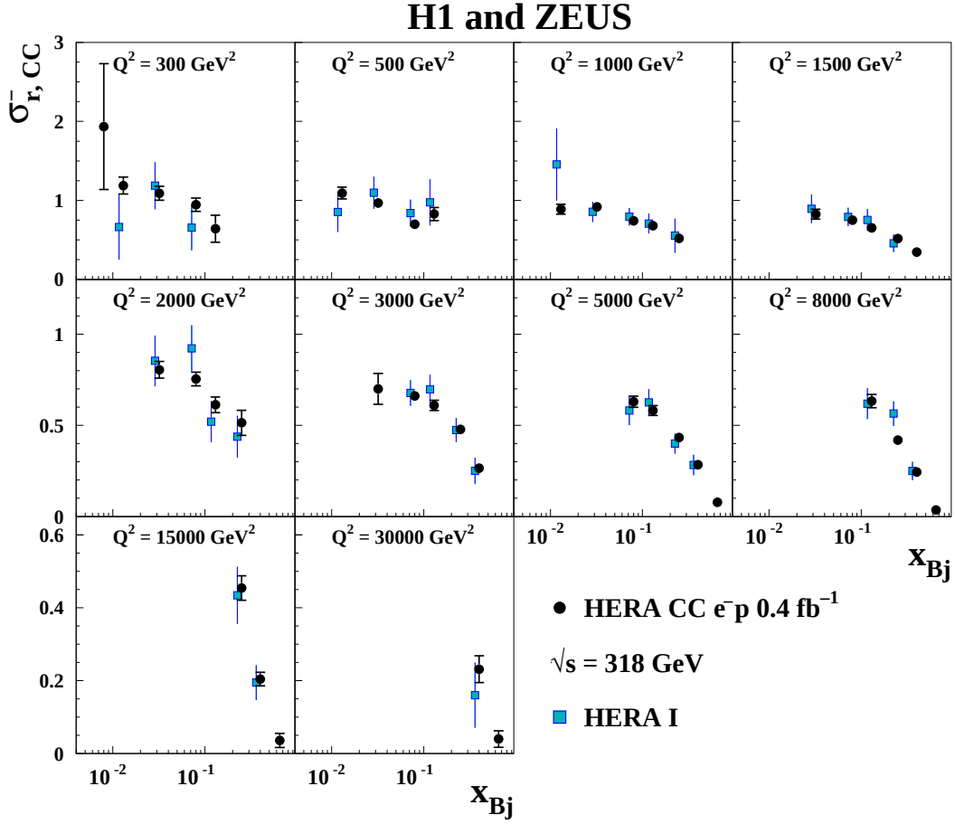
Figure 15: The combined HERA data for the inclusive CC e^-p reduced cross sections as a function of x_{Bj} for the 10 different values of Q^2 compared to the results from HERA I alone [2]. The individual measurements are displaced horizontally for better visibility. Error bars represent the total uncertainties.
