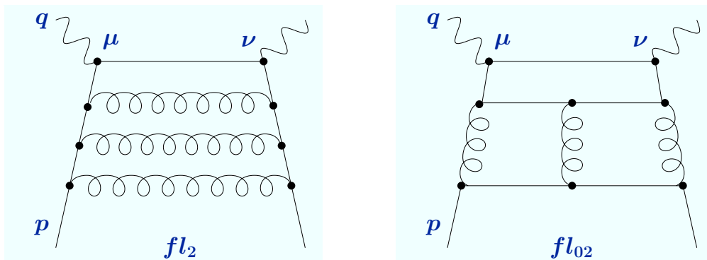
Figure 1: Typical third-order Feynman diagrams for the two flavour classes contributing to quark-initiated charged-current DIS. Depending on the structure function, the boson lines at the top are replaced by \varepsilon_{pq\mu\nu} or a combination of g_{\mu\nu} and p_\mu p_\nu , and the quark lines at the bottom by \gamma_p or \gamma_p \gamma_5 (in Schoonship notation). The vertices with \mu and \nu represent vector or axial-vector couplings.
