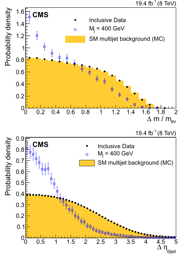
Fig. 2. Probability density distributions of \Delta m / m_{\text{av}} (top) and \Delta\eta_{\text{dijet}} (bottom) for events from data, the simulated SM multijet sample, and a 400 GeV top squark signal. Statistical uncertainties are shown for the top squark signal as vertical bars and for data as arrows. Events contain at least four jets, each with p_T > 120 GeV and |\eta| < 2.5 , and all distributions have an area normalized to unity.
