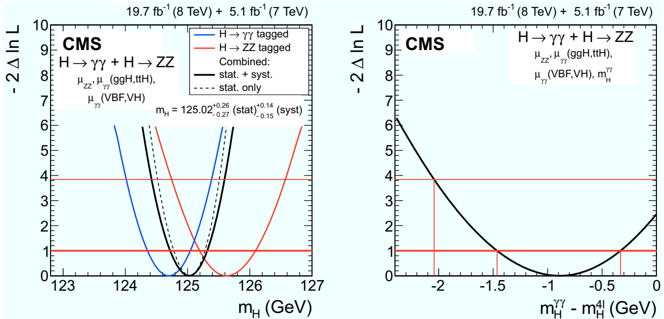
Fig. 2 (Left) Scan of the test statistic q(m_H) = -2\Delta\ln\mathcal{L} versus the mass of the boson m_H for the H \rightarrow \gamma\gamma and H \rightarrow ZZ \rightarrow 4\ell final states separately and for their combination. Three independent signal strengths, (ggH, ttH) \rightarrow \gamma\gamma , (VBF, VH) \rightarrow \gamma\gamma , and pp \rightarrow H \rightarrow
