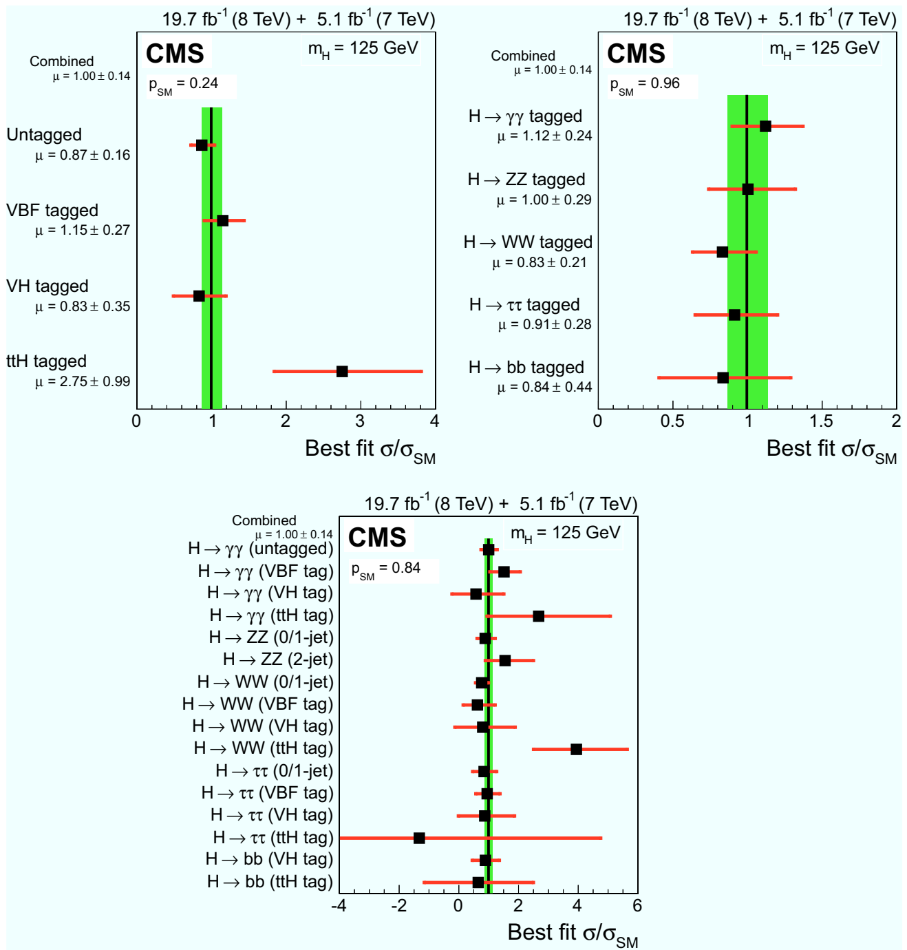
Fig. 4 Values of the best-fit \sigma/\sigma_{SM} for the overall combined analysis (solid vertical line) and separate combinations grouped by production mode tag, predominant decay mode, or both. The \sigma/\sigma_{SM} ratio denotes the production cross section times the relevant branching fractions, relative to the SM expectation. The vertical band shows the overall \sigma/\sigma_{SM} uncertainty. The horizontal bars indicate the \pm 1 standard deviation uncertainties in the best-fit \sigma/\sigma_{SM} values for the individual combinations; these bars include both statistical and systematic uncertainties.
