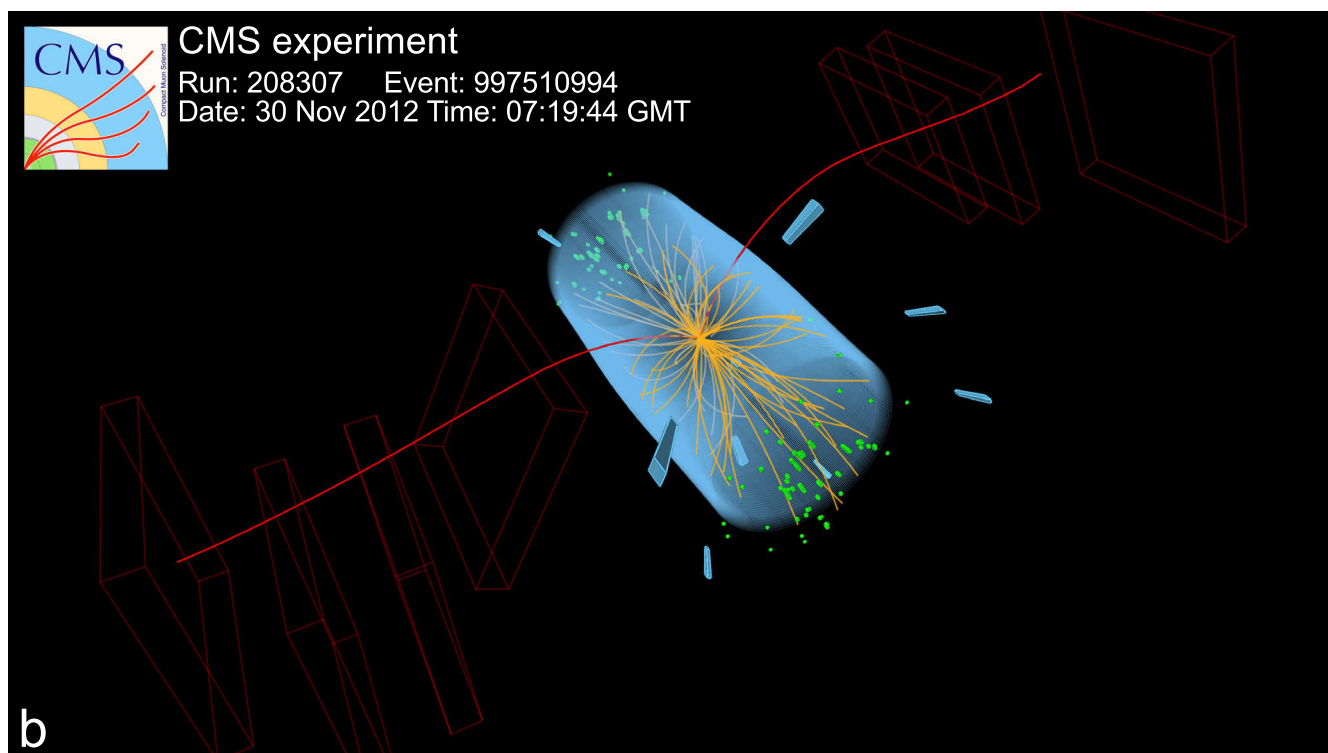
Extended Data Figure 3 | Schematic of the CMS detector and event display for a candidate B_s^0 \rightarrow \mu^+ \mu^- decay at CMS. a , The CMS detector and its components; see ref. 20 for details. b , A candidate B_s^0 \rightarrow \mu^+ \mu^- decay produced
