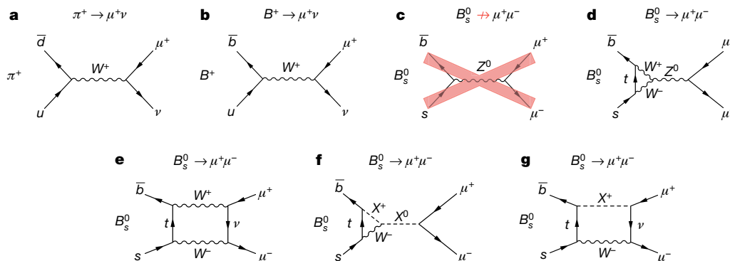
Figure 1 | Feynman diagrams related to the B^0_s \rightarrow \mu^+ \mu^- decay. a , \pi^+ meson decay through the charged-current process; b , B^+ meson decay through the charged-current process; c , a B^0_s decay through the direct flavour changing neutral current process, which is forbidden in the SM, as indicated by a large red
