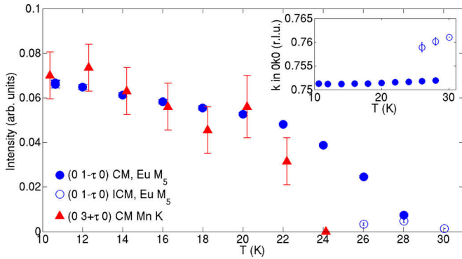
FIG. 2. (Color online) Temperature dependence of the integrated intensity of the C type (0\ 1 - \tau\ 0) reflection at the Eu M_5 resonance (blue circles). Red triangles show the T dependence of the C type (0\ 3 + \tau\ 0) reflection at the Mn K edge. The data have been scaled to fit onto the same plot. The inset shows the peak positions in q space over the same temperature range.
