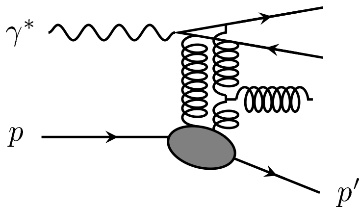
Figure 17: On of diagrams of q\bar{q}g production in the Two-Gluon-Exchange model.
