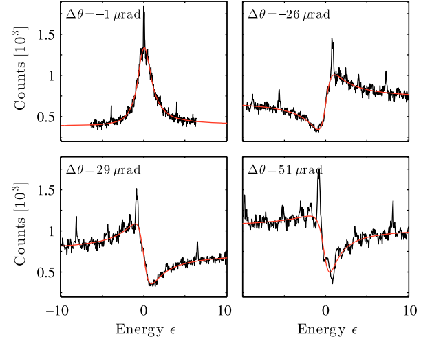
FIG. 2 (color online). Fano line shape control with nuclei. The different panels show the reflected intensity measured at different relative incidence angles \Delta\theta = \theta - \theta_{\min} with uncertainty \pm 3 \mu\text{rad} . Experimental data are shown without baseline subtraction. Therefore, the intensities in the different panels cannot be directly compared.
