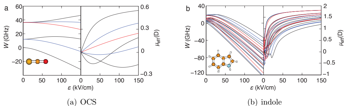
Figure 2. Stark energies W (left plots) and effective dipole moments \mu_{\text{eff}} (right plots) of (a) the linear-top molecule OCS and (b) the asymmetric-top molecule indole ( C8NH7 ) for the M = 0 (black), M = 1 (blue), and M = 2 (red) levels of all \tilde{J} = 0-2 states. All data was calculated using CMlStark [96]. See text for details.
