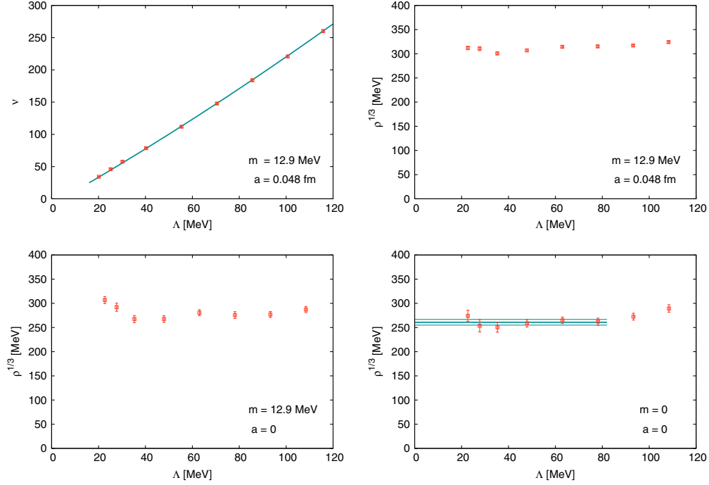
FIG. 1 (color online). Top-left: The mode number as a function of \Lambda for O7; a quadratic fit of the data ( \Lambda in MeV) gives \nu = -9.0(13) + 2.07(7)\Lambda + 0.0022(4)\Lambda^2 . Top-right: \tilde{\rho}^{1/3} for the same ensemble as a function of \Lambda = (\Lambda_1 + \Lambda_2)/2 . Bottom-left: \tilde{\rho}^{1/3} in the continuum limit at the smallest reference quark mass. Bottom-right: \tilde{\rho}^{1/3} in the continuum and chiral limit. Note the flat dependence on \Lambda which agrees with the expectation from NLO ChPT; a plateau fit in the interval 20–80 MeV is also shown.
