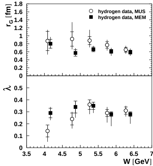
Fig. 5. Parameter r_G and \lambda as a function of W , obtained with MEM and MUS methods on hydrogen. The inner and outer error bars indicate the statistical and total uncertainties. For the latter the statistical and systematic uncertainties are added in quadrature.
