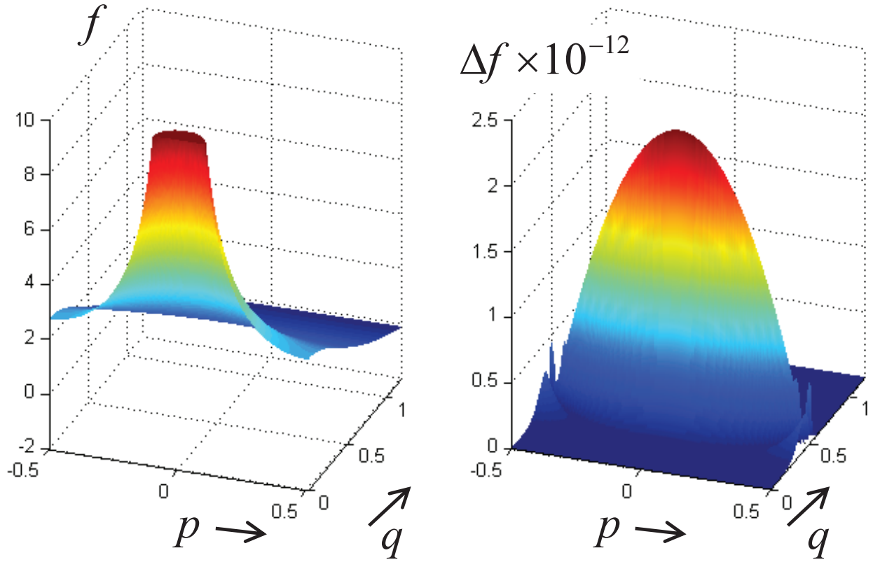
FIG. 3: Function f(p, q, 0) and absolute error \Delta f(p, q, 0) of the numerical calculation. As f is singular at the origin ( p = q = 0 ), it is truncated for the plot to values below 10. The transition from the Taylor approximation (for small |q| ) to the Fourier series is at |q| = 0.5 . The Taylor approximation is used for the upper part of the sum from M_t = 16 to infinity. The harmonic expansion is truncated after 8 terms.
