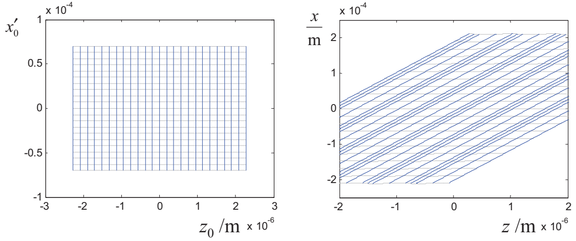
FIG. 15: Application C: visualization of transport transformation of (z_0, x'_0) , after laser heater undulator to (x, z) , at 15.5 m position for particles without offset x_0 .
