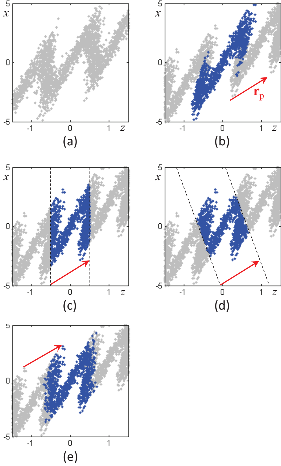
FIG. 1: Periodic particle distributions and periodic shift vector \mathbf{r}_p : (a) pseudo-periodic random distribution with periodic behavior; (b) generating set S_p and periodically repeated particles in blue resp. gray; (c) equivalent generating set in slice volume between two planes shifted by \mathbf{r}_p ; (d) other equivalent set in different volume slice; (e) equivalent generating set without sharp truncation.
