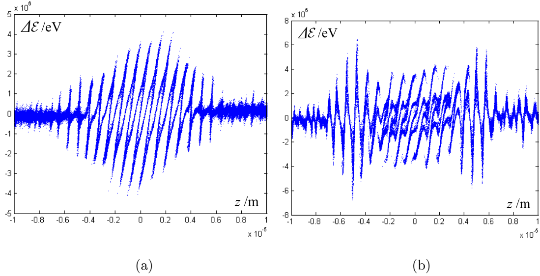
FIG. 8: Application A: longitudinal phase space (a) direct after chicane 3 and (b) 15 m behind, for 30 fs (FWHM) laser modulation, calculated with 1E6 macro-particles, by QField.
