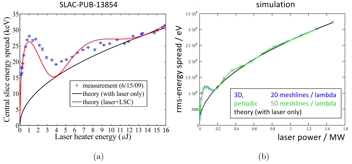
FIG. 22: (a) Measurement [10], (b) simulation with QField-periodic and QField-non-periodic.
