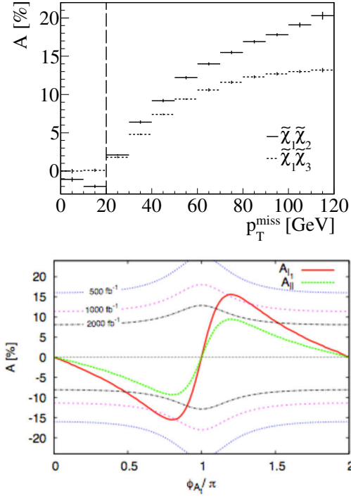
Fig. 145 Top panel: p_T^{\text{miss}} dependence of CP asymmetries in neutralino-pair production and decay processes (from [1070]). Bottom panel: Asymmetries, A_{\ell_1} and A_{\ell\ell} as functions of \Phi_{A_\ell} (from [1141]).
