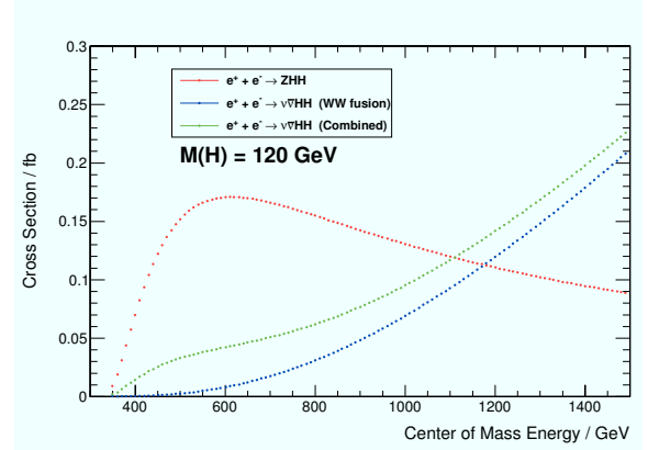
Fig. 47 Cross sections for the double Higgs production processes, e^+e^- \rightarrow Zhh and e^+e^- \rightarrow \nu\bar{\nu}hh , as a function of \sqrt{s} for m_h = 120 GeV.
