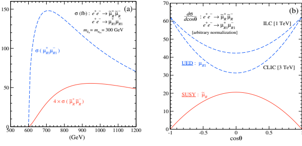
Fig. 132 The threshold excitation (a) and the angular distribution (b) in pair production of smuons in the MSSM, compared with the first spin-1/2 Kaluza-Klein muons in a model of universal extra dimensions; for details, see Ref. [1076].
