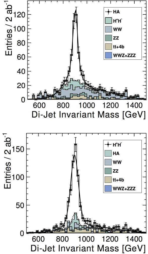
Fig. 13 Upper plot: Reconstructed 2-jet invariant mass for associated production: e^+e^- \rightarrow AH \rightarrow bbbb for a Higgs mass of 900 GeV at a collider energy of 3 TeV; lower plot: Similar plot for e^+e^- \rightarrow H^+H^- \rightarrow t\bar{t}b\bar{b} .
