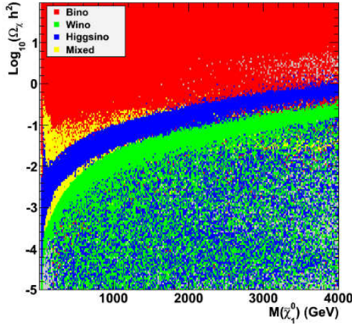
Fig. 122 Neutralino relic density as a function of the neutralino LSP mass from a scan of the pMSSM parameter space. The colours indicate the nature of the neutralino LSP with the largest occurrence in each bin.
