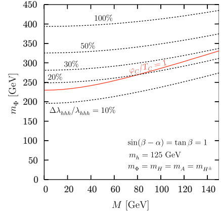
Fig. 71 Contour plots of the deviation in the hhh coupling in the (m_\phi, M) plane for m_h = 125 GeV and \sin(\beta - \alpha) = 1 . The red line indicates \phi_c/T_c = 1 , above which the strong first order phase transition occurs ( \phi_c/T_c > 1 ) [337].
