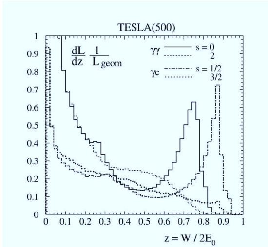
Fig. 96 The distribution of \gamma\gamma and e\gamma center-of-mass energy W with respect to the e^+e^- energy ( 2E_0 ) from simulation of the PLC luminosity spectra [544]. Contributions of various spin states of produced system are shown.
