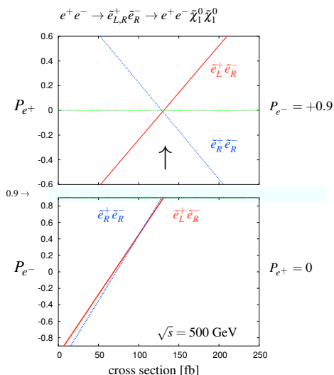
Fig. 5 Polarized cross sections versus P_{e^-} (bottom panel) and P_{e^+} (top panel) for e^+e^- \rightarrow \tilde{z}\tilde{e} -production with direct decays in \tilde{\chi}_1^0 e in a scenario where the non-coloured spectrum is similar to a SPS1a-modified scenario but with m_{\tilde{e}_L} = 200 GeV, m_{\tilde{e}_R} = 195 GeV. The associated chiral quantum numbers of the scalar SUSY partners \tilde{e}_{L,R} can be tested via polarized e^\pm -beams.
