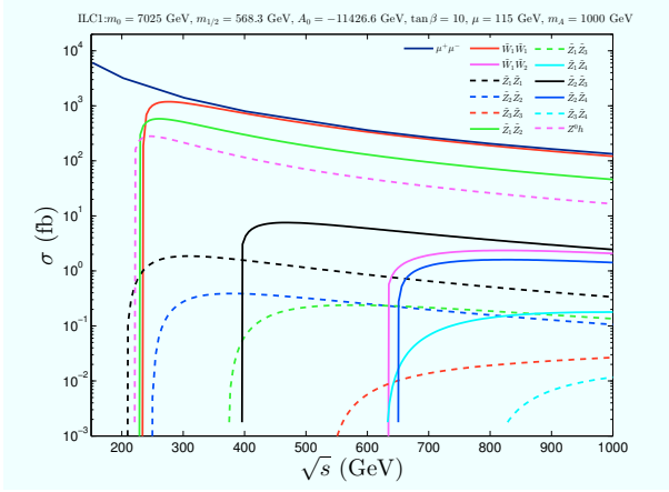
Fig. 128 Sparticle production cross sections vs. \sqrt{s} at a Higgsino factory for a radiatively-driven natural SUSY benchmark point [969].
