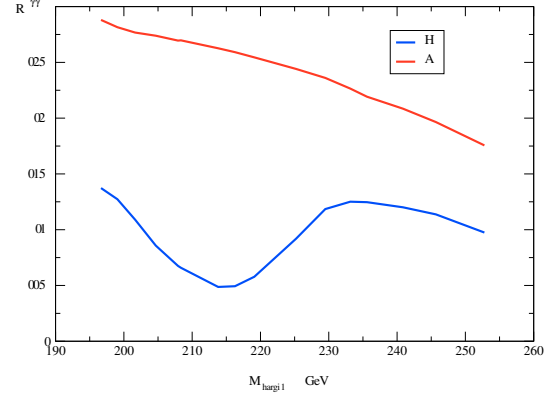
Fig. 90 The reduced coupling R^{\gamma\gamma} , as defined in Eq. (81), as function of M_{\text{chargino}_1} for M_{A_5} \sim M_{H_5} \sim 260 GeV, for a scenario explaining a 130 GeV photon line from dark matter annihilation in the galactic center.
