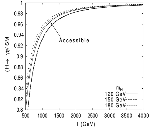
Fig. 98 Ratio \frac{\Gamma(h \rightarrow \gamma\gamma)}{\Gamma(h \rightarrow \gamma\gamma)^{\text{SM}}} as a function of the mass scale of the new physics f in the Littlest Higgs model [467], for different Higgs boson masses. “Accessible” indicates the possible variation of the rate for fixed f .
