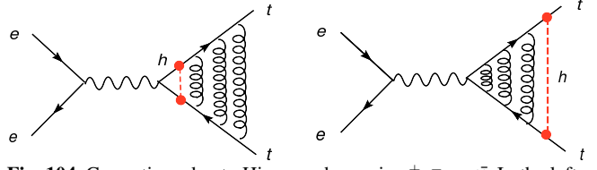
Fig. 104 Corrections due to Higgs exchange in e^+e^- \rightarrow t\bar{t} . In the left diagram the Higgs exchange contributes to the production vertex for \gamma\bar{t}t, Z\bar{t}t , which occurs at short distance when the t\bar{t} -pair is separated by r \sim 1/m_t . In the right diagram Higgs exchanges occurs after bound-state formation between top and anti-top quarks separated by the scale of the bound-state r \sim 1/(m_t\alpha_s) .
