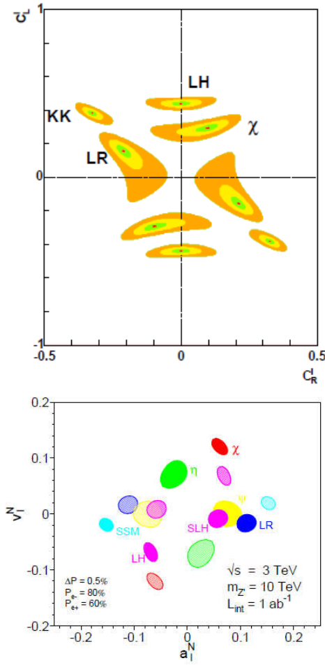
Fig. 121 Top: Resolving power (95% CL) for M_{W'} = 1, 1.5, \text{ and } 2 \text{ TeV} and \sqrt{s} = 500 \text{ GeV} , \mathcal{L}_{\text{int}} = 1 \text{ ab}^{-1} , |P_{e^-}| = 80\% , |P_{e^+}| = 60\% , for leptonic couplings based on the leptonic observables \sigma , A_{\text{LR}} , A_{\text{FB}} . The couplings correspond to the E_6 \chi , LR, LH, and KK models. From Ref. [905]. Bottom: Expected resolution at CLIC with \sqrt{s} = 3 \text{ TeV} and \mathcal{L} = 1 \text{ ab}^{-1} on the "normalised" leptonic couplings of a 10 \text{ TeV} Z' in various models, assuming lepton universality. The mass of the Z' is assumed to be unknown. The couplings correspond to the E_6 \chi , \eta , and \psi , the SSM, LR, LH and SLH models. The couplings can only be determined up to a twofold ambiguity. The degeneracy between the \psi and SLH models might be lifted by including other channels in the analysis ( t\bar{t} , b\bar{b} , ...). From Refs. [9, 906].
