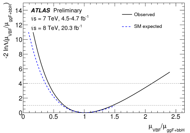
Fig. 19 Likelihood for the ratio \mu_{VBF}/\mu_{ggF+bbH} obtained by ATLAS for the combination of the H \rightarrow \gamma\gamma , ZZ \rightarrow 4\ell and WW \rightarrow 2\nu 2\ell channels and m_H = 125.5 \text{ GeV} [105].
