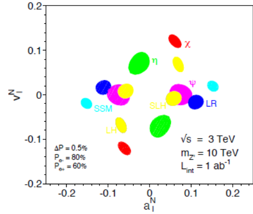
Fig. 10 New gauge bosons in the \mu^+\mu^- channel. The plot shows the expected resolution at CLIC with \sqrt{s} = 3 TeV and \mathcal{L} = 1 \text{ab}^{-1} on the ‘normalized’ vector v_f^N = v_f \sqrt{s/(m_{Z'}^2 - s)} and axial-vector a_f^N = a_f \sqrt{s/(m_{Z'}^2 - s)} couplings to a 10 TeV Z' in terms of the SM couplings v_f, a_f . The mass of Z' is assumed to be unknown, nevertheless the couplings can be determined up to a two-fold ambiguity. The colours denote different Z' models [9].
