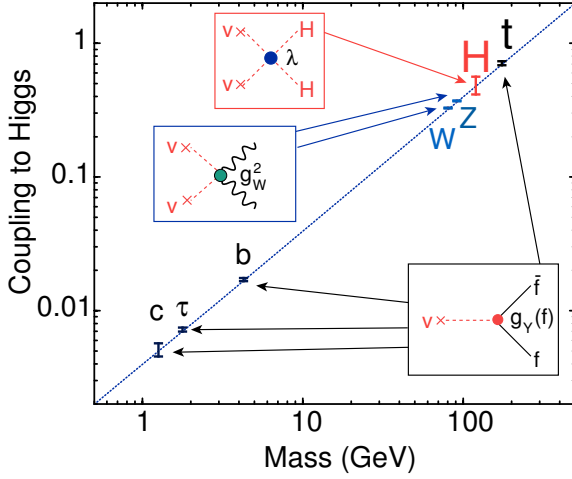
Fig. 39 Mass-coupling relation [136].
