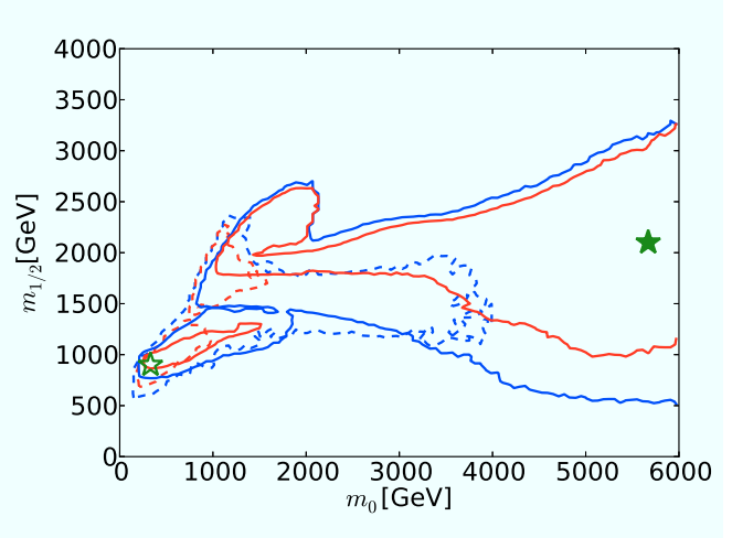
Fig. 155 The (m_0, m_{1/2}) planes in the CMSSM including the ATLAS 20/fb jets + \bar{E}_T , BR(B_{s,d} \rightarrow \mu^+ \mu^-) , m_h , \Omega_\chi h^2 , LUX, and other constraints. The most recent results are indicated by solid lines and filled stars, and previous fit based on \sim 5/\text{fb} of LHC data is indicated by dashed lines and open stars. The blue lines denote 68% CL contours, and the red lines denote 95% CL contours.
