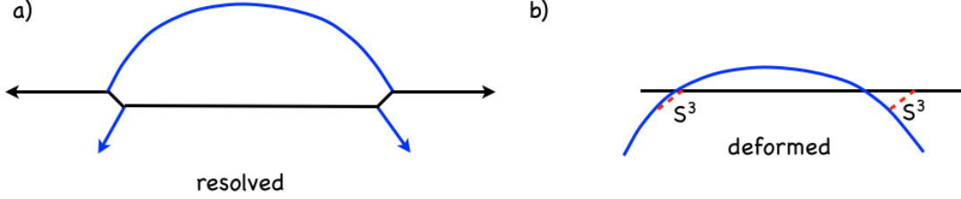
Figure 6: (a) Web diagram for the resolved 2-conifold geometry of Aganagic et al. [37]. (b) The deformed version of (a) after the geometric transition.
