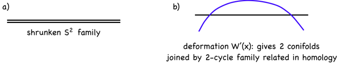
Figure 5: (a) Web diagram for the initial curves-of-conifolds geometry of Aganagic et al. [37]. (b) The deformation W'(x) leading to two conifolds connected by a 2-cycle family related in homology.
