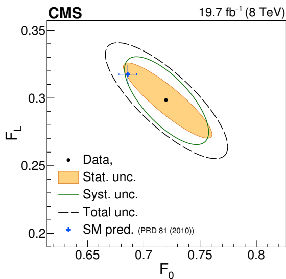
Figure 2. Combined results from the muon+jets and electron+jets events for the left-handed and longitudinal W boson helicity fractions, shown as 68% contours for statistical, systematic, and total uncertainties, compared with the SM predictions [10].
