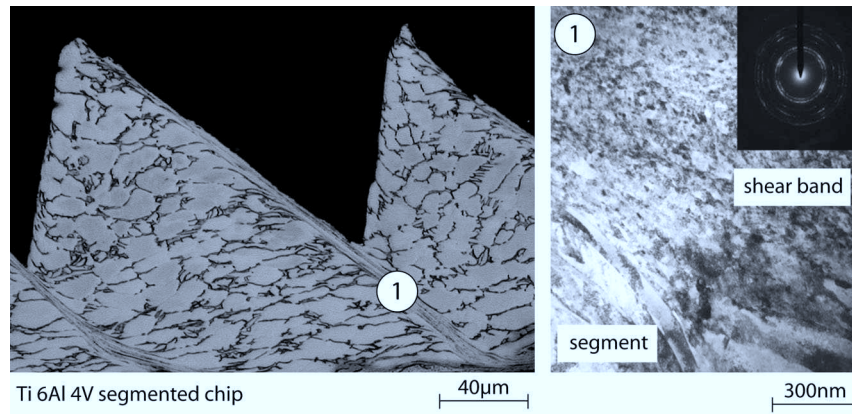
FIG. 3. Imaging the localized shear band. (Left panel) Optical microscopy image of a Ti6Al4V segmented chip produced in orthogonal high-speed cutting at v_c = 10 m/s; a_p = 0.1 mm. The average \alpha grain size in the segments is 20\text{ }\mu\text{m} . (Right panel) Detail from position 1 showing that the shear band consists of equiaxed, nanocrystalline \alpha grains. The average grain size is about 10\text{ nm} . The shear band can be clearly distinguished from the segment. The SAD (inset) shows that a metastable \beta phase is not present. Supplemental Material [8], Fig. 6 shows the same behavior in a \beta -Ti alloy.
