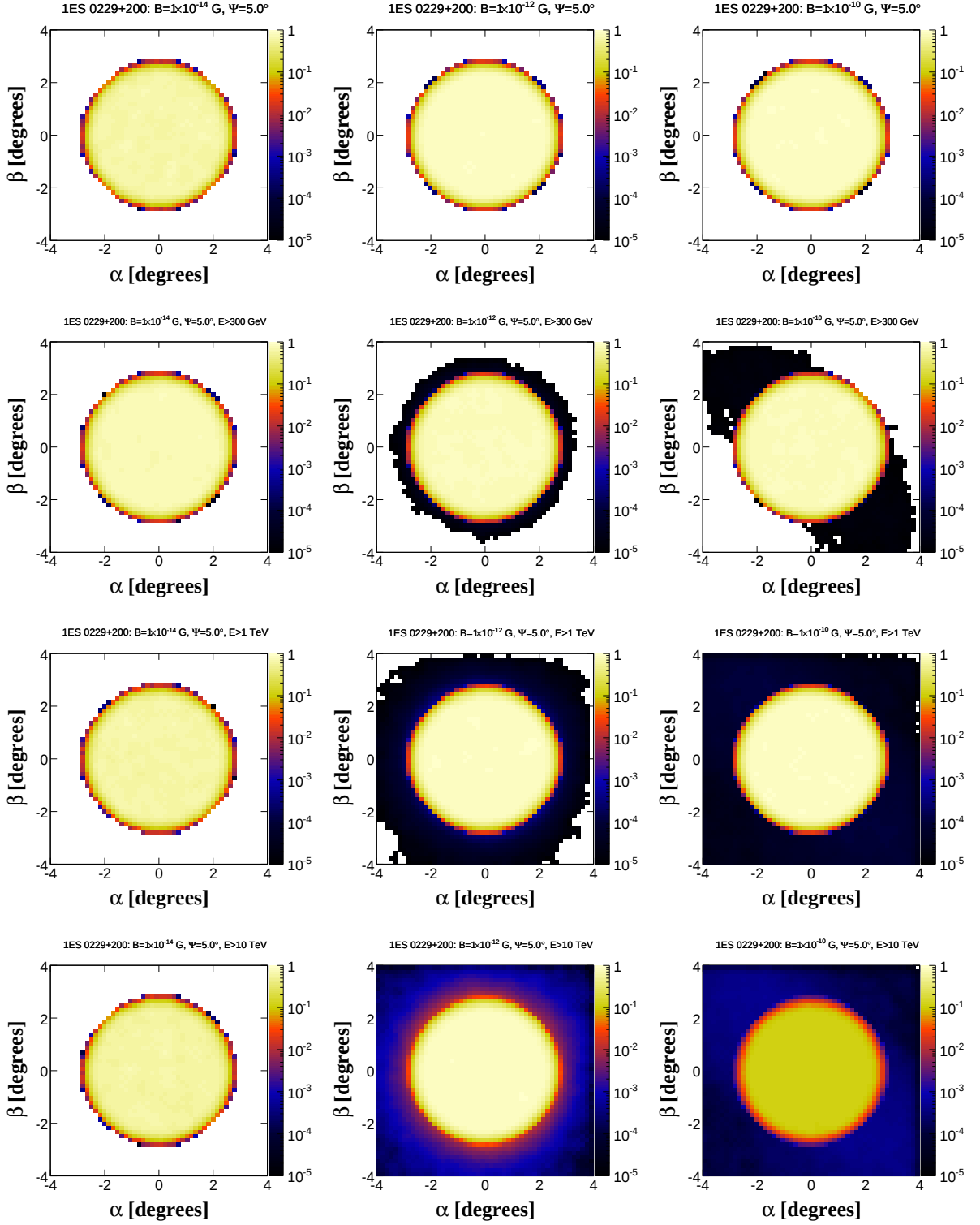
Figure 9.3: Simulated pair halos for 1ES 0229+200 for three magnetic field strengths 10^{-14} G (left column), 10^{-12} G (middle column), 10^{-10} G (right column), for the following energy ranges: E > 10 GeV, E > 300 GeV, E > 1 TeV and E > 10 TeV (from top to bottom). The color scale indicates the number of events per bin, where each bin has a size of approximately 0.1^\circ .
