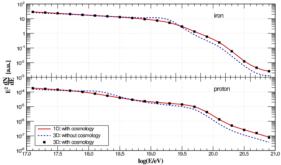
Figure 7.7: Spectra for the 1D simulation (solid line), the 3D without cosmology (dashed line) and the 3D corrected for cosmology (squares) for the a pure iron (top) and pure proton (bottom) composition. The spectra are normalized to the total number of events times 100 for iron, and 0.01 for proton.
