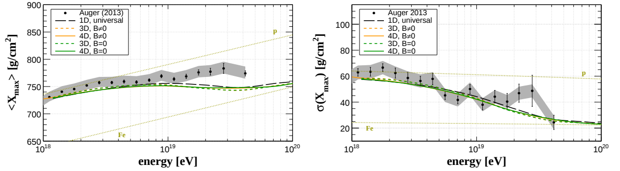
Figure 7.15: Inferred \langle X_{\text{max}} \rangle and \sigma(X_{\text{max}}) for the different scenarios. The hadronic interaction model considered is EPOS-LHC.
