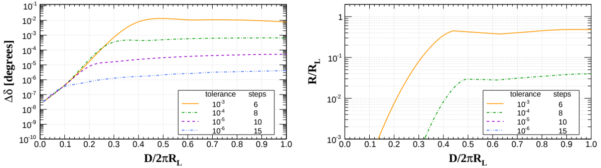
Figure 5.3: Directional (left panel) and positional (right) errors, as a function of the propagated distance ( D ) in units of Larmor length ( 2\pi R_L ). Here \Delta\delta designates the error in the deflection, and R = |\vec{R}| the position. In the plots the number of steps required to achieve the results with the required tolerance are also indicated. In the right panel the curves for tolerances of 10^{-5} and 10^{-6} cannot be seen, although they are indicated in the legend, because they are below 10^{-12} in the whole interval displayed.
