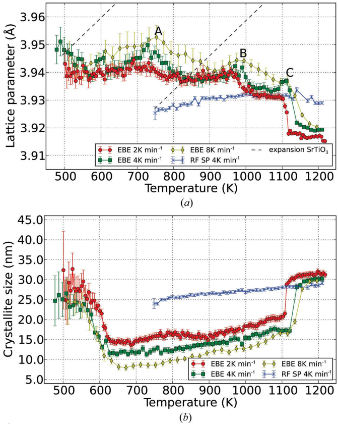
Figure 3 Temperature dependence of (a) lattice parameter and (b) crystallite size of SrTiO 3 extracted from in situ GI-XRD with different temperature ramps of 2, 4 and 8 K min -1 for Sr-rich (EBE) and 4 K min -1 for Sr-depleted layers (RF SP), determined by Rietveld refinement using TOPAS . Dashed lines highlight the relative thermal lattice expansion calculated from the SrTiO 3 thermal expansion coefficient (de Ligny & Richet, 1996). Prominent points in the development of the EBE samples' crystallization are highlighted by the letters A, B and C.
