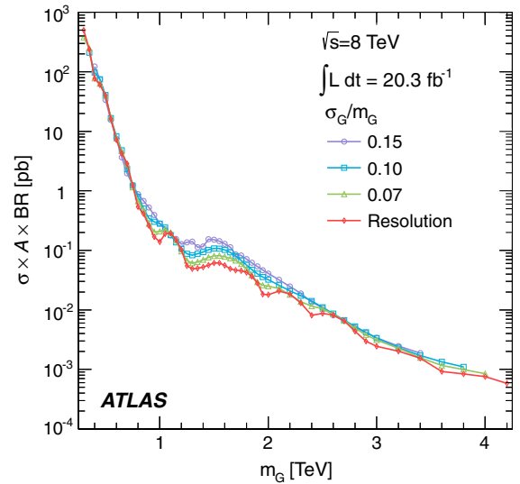
FIG. 8 (color online). The 95% C.L. upper limits on \sigma \times \mathcal{A} for a simple Gaussian resonance decaying to dijets as a function of the mean mass, m_G , for four values of \sigma_G/m_G , taking into account both statistical and systematic uncertainties.
