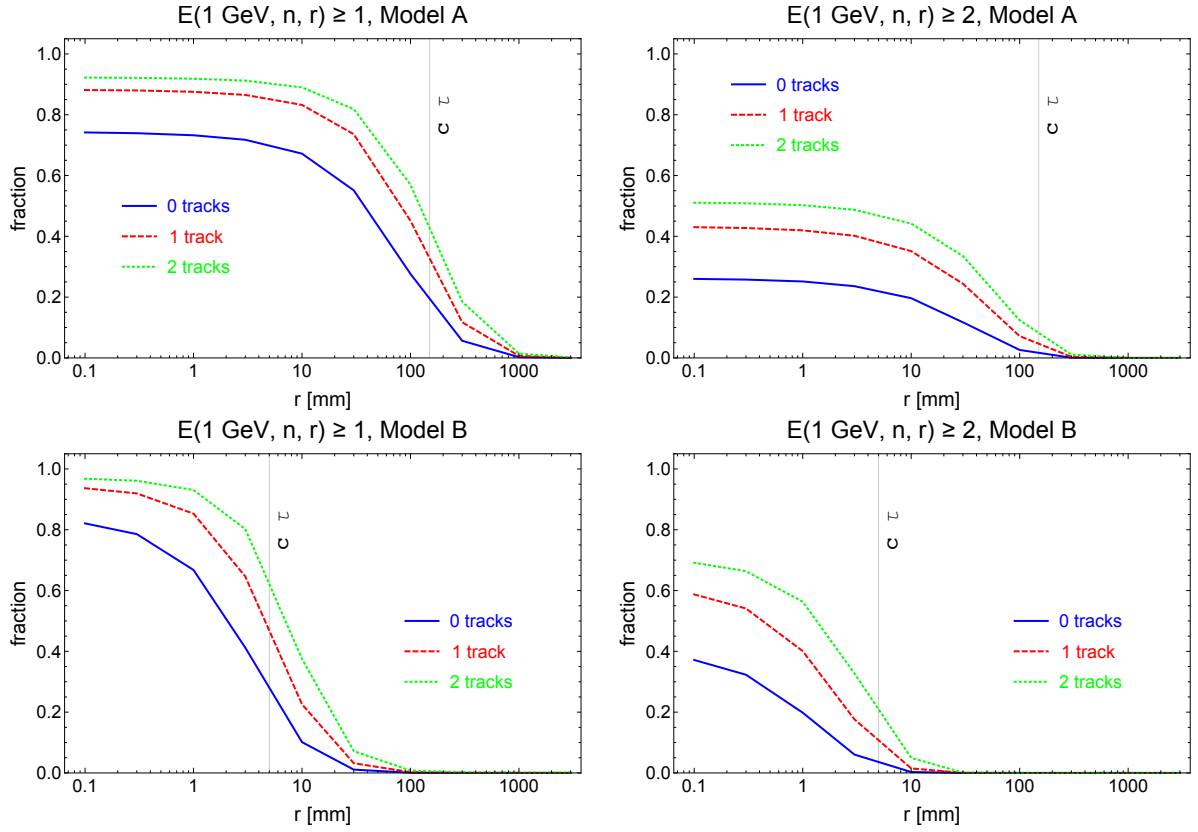
Figure 8: Fraction of signal events in model A (top) and model B (bottom) which have at least one (left) or two (right) emerging jets with p_T^{\min} = 1 \text{ GeV} as a function of r , the transverse distance. Within each plot, the curves are a maximum of 0, 1, and 2 tracks with transverse origin less than r going from bottom to top. A vertical line is put at the proper lifetime of the particular model. All events must pass the kinematic preselection cuts.
