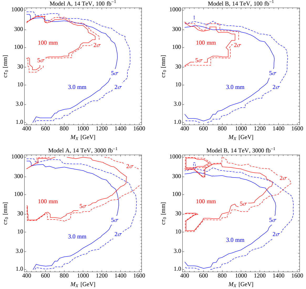
Figure 10: Region of lifetime and mediator mass parameter space probed with 100 fb -1 (top row) and 3000 fb -1 (bottom row) at the 14 TeV LHC. For each model we show 2σ (dashed) and 5σ contours (solid) in the M_X - c\tau_0 plane, assuming a systematic uncertainty of 100% on the background. The different colors correspond to requiring E(1 \text{ GeV}, 0, 3 \text{ mm}) \geq 2 (blue) and E(1 \text{ GeV}, 0, 100 \text{ mm}) \geq 2 (red).
