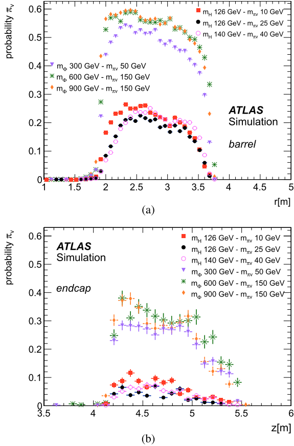
Fig. 1. The probability ( \varepsilon_{\pi_v} ) for a single \pi_v to pass the trigger as a function of the \pi_v (a) radial decay length in the barrel and (b) the z position of the decay vertex in the endcaps for several \Phi and \pi_v masses.
