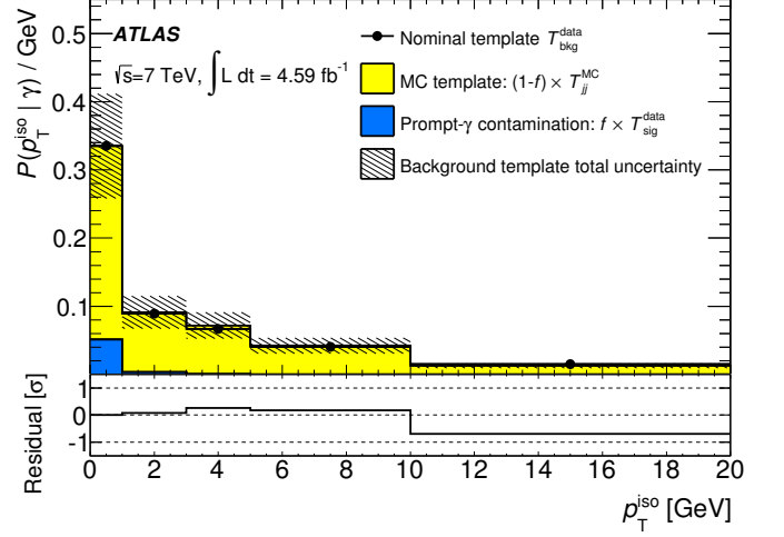
Figure 5: Track-isolation background template distribution after maximization of the likelihood L_f defined in Eq. 3 (top) and normalized residuals (bottom). The markers correspond to the nominal hadron background template. The stacked filled histograms represent the fraction of prompt photons in the hadron-fake control region (obtained as f \times T_{\text{sig}}^{\text{data}} ) and the fraction of hadron-fakes (obtained from the simulation-based template as (1-f) \times T_{jj}^{\text{MC}} ) as given by the fit. The normalized residuals, shown in the bottom plot, are defined as the difference between the ‘Nominal template’ and the sum of (1-f) \times T_{jj}^{\text{MC}} and f \times T_{\text{sig}}^{\text{data}} , divided by the total uncertainty \sigma_{\theta} . The last bin contains any overflow.
