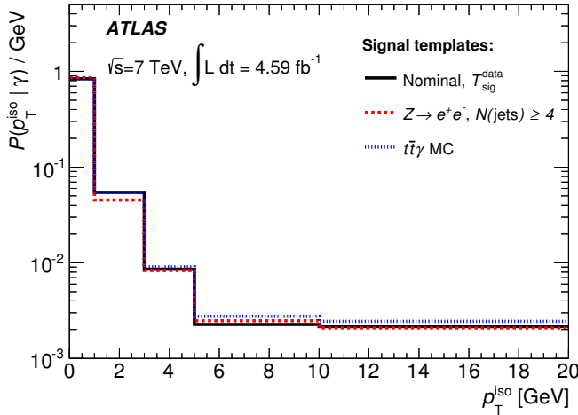
Figure 3: Comparison of the nominal prompt-photon track-isolation ( p_{\text{T}}^{\text{iso}} ) template with the template obtained from data using a Z(\rightarrow e^+e^-) + \geq 4 -jets selection, and with the template obtained from t\bar{t}\gamma simulation. The distributions show the probability P(p_{\text{T}}^{\text{iso}}|\gamma) of observing a photon in a given p_{\text{T}}^{\text{iso}} bin per GeV. The last bin contains any overflow.
