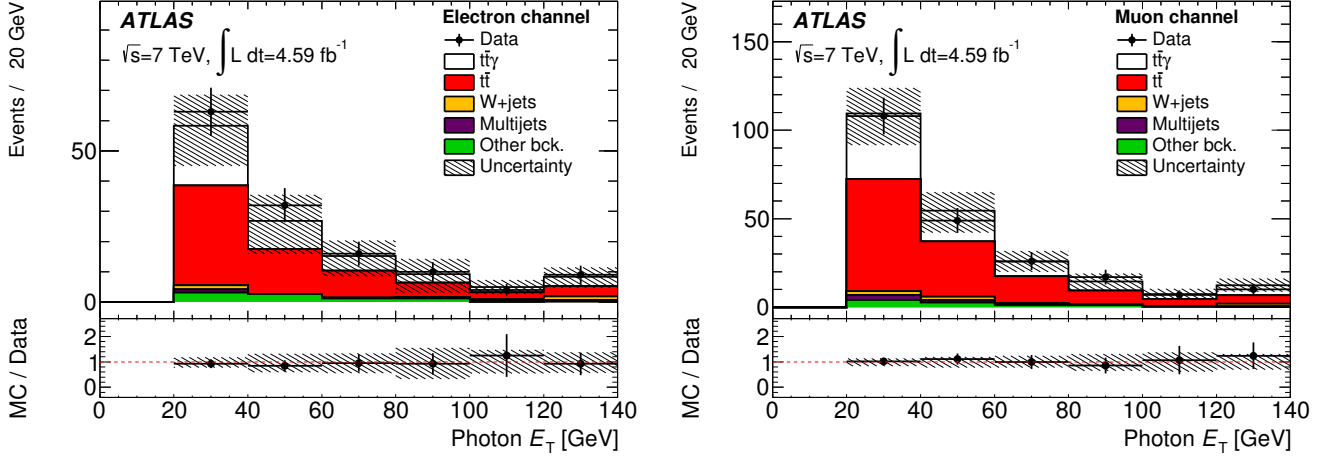
Figure 2: Distributions for the t\bar{t}\gamma selection (see text). The photon candidate transverse momentum ( E_T ) distribution in data (points) is compared to the expectation (stacked histograms) for the electron (left) and muon (right) channels. The contribution from multijet+ \gamma production and its uncertainties are estimated using a data-driven technique (see Sec. VII B). The remaining contributions are estimated using Monte Carlo simulation. Other backgrounds (labeled as ‘Other bck.’) include contributions from Z + jets, dibosons and single top. The contribution from t\bar{t} production with prompt photons (labeled as ‘ t\bar{t}\gamma ’) is estimated using the WHIZARD t\bar{t}\gamma Monte Carlo simulation. The contribution from t\bar{t} events with electrons and hadrons misidentified as prompt photons is obtained using inclusive t\bar{t} Monte Carlo simulation. The uncertainty band includes statistical and systematic uncertainties. The systematic uncertainties include those on photon, lepton, jet, E_T^{\text{miss}} , and b -tagging modeling, as well as systematic uncertainties for the multijet background estimate. The last bin contains any overflow.
