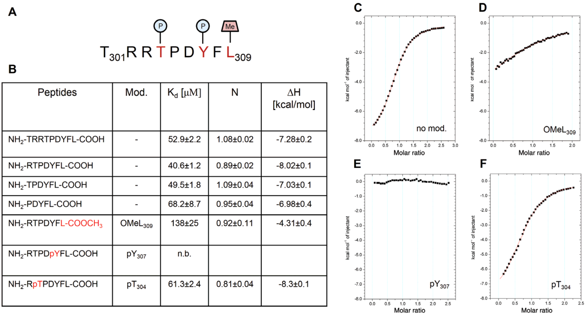
Figure 1 Interaction of PTPA with the C-terminal peptide of the catalytic subunit of PP2A. (A) Sequence and known modifications of the invariant C-terminus of the catalytic subunit. (B) Resulting binding properties of peptides of various lengths and with different modifications to PTPA are shown. (C–F) Integrated heat changes upon binding of peptides with different modifications (shown in the different panels) to PTPA are plotted against the peptide/PTPA concentration ratio. n.b., no binding detected.
