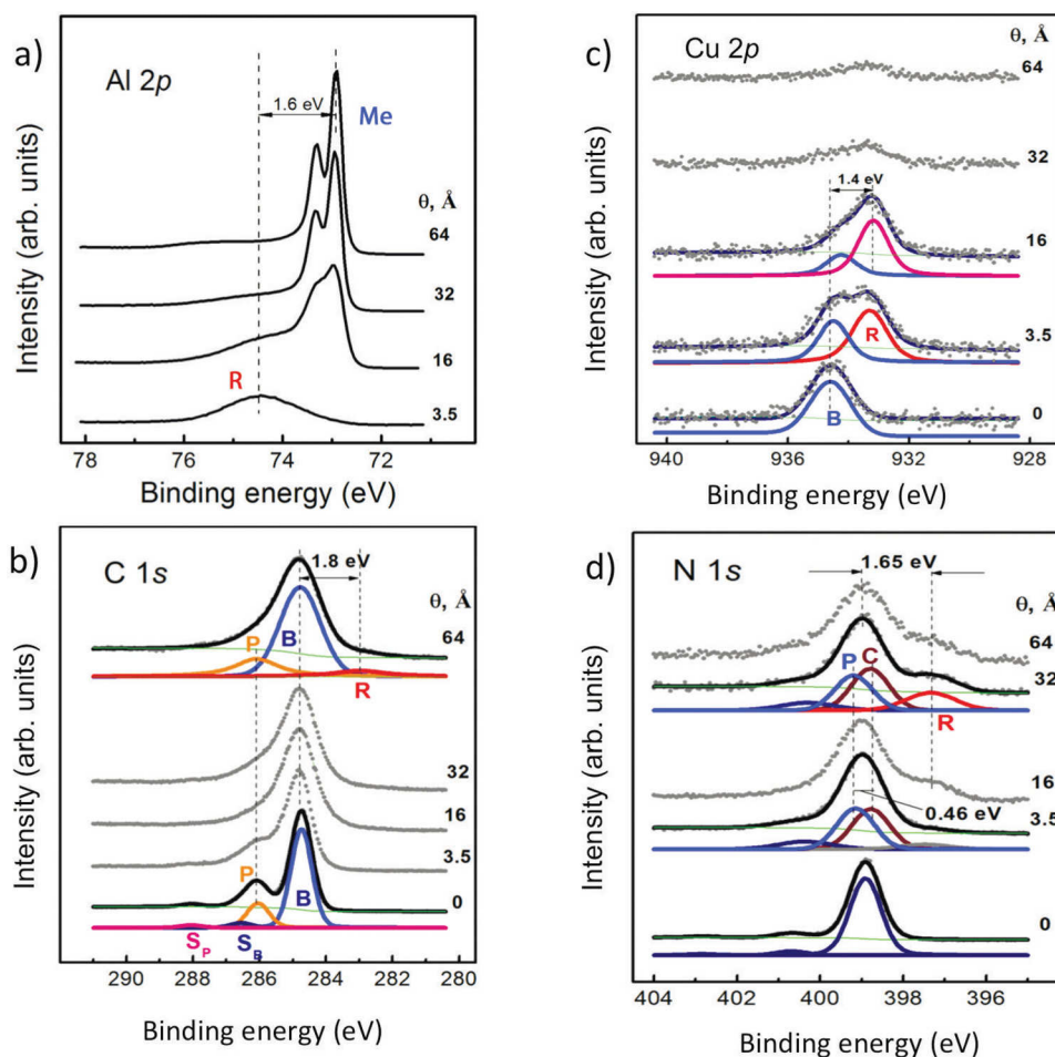
FIG. 4. CL normalized photoemission spectra as a function of Al deposition on CuPc thin films at room temperature (RT): Al 2 p (a), C 1 s (b), Cu 2 p (c), and N 1 s (d). The nominal coverage of the Al deposition is indicated. The behavior of Cu 2 p CL is similar to what has been observed for the case of Li, Fe, and Co deposition onto CuPc (see below in text).
