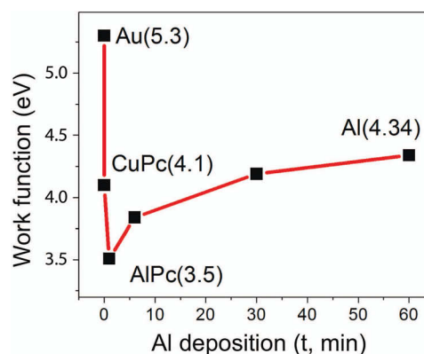
FIG. 5. Work function changes induced by Al deposition on CuPc thin films at RT, determined from PES data using the cut-off procedure.
