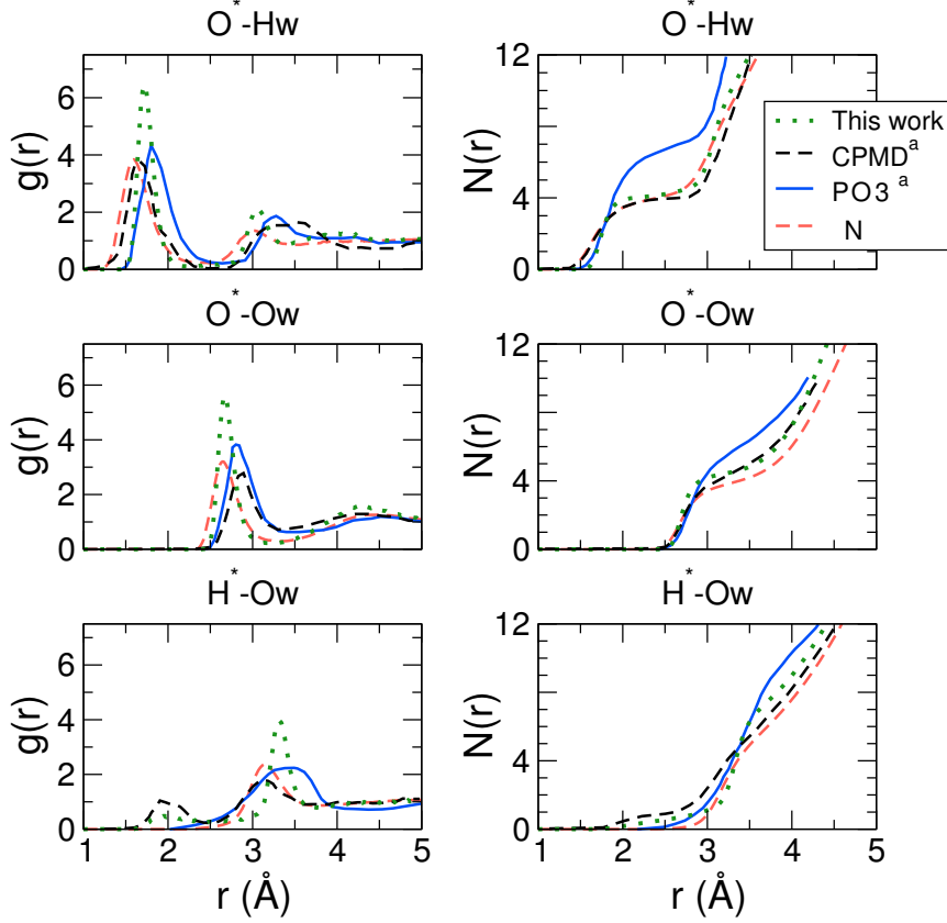
Figure S5: Hydroxide-water radial distribution functions. The standard g(r) and cumulative N(r) radial distribution functions of water oxygen Ow and hydrogen Hw around the hydroxide oxygen O* and hydrogen H*. The CPMD and POL3 data are obtained from Bucher et al. [38], and the RING model data from Ufimtsev et al. [52].
