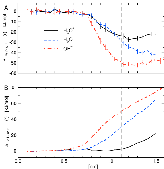
Figure 4: Decomposition of enthalpy (3B) into interaction energies for each of three solutes as a function of distance r from the droplet center (visualized in 1). The grey dashed line indicates the Gibbs dividing surface.
