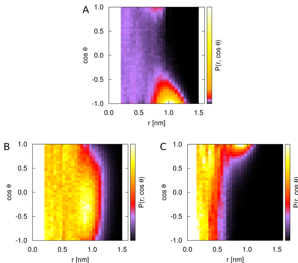
Figure 5: Orientation distribution for A) hydronium, B) water and C) hydroxide in a water droplet as a function of distance from the center of the droplet r , as in 1A. \theta is the angle between the dipole vector of the solute and the vector from the center of the droplet to the oxygen atom of the solute.
