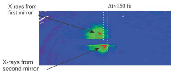
Figure 15. Image of the Ti:sapphire laser light transmitted through a thin \text{Si}_3\text{N}_4 membrane when illuminated with two x-ray pulses separated by \sim 150 fs from the soft XRSF unit. Transmission of the 800 nm light through the film increases in areas illuminated by x-rays, spatially encoding the arrival time of the x-rays relative to the laser pulse in the horizontal direction.
