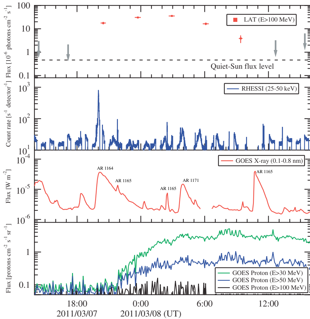
Figure 1. Multi-wavelength and proton light curves of GOES M3.7 SOL2011-03-07T20:12. \gamma -ray data are from the Fermi LAT, HXR from RHESSI , and soft X-rays and protons from GOES . Vertical error bars of LAT data indicate 1\sigma statistical uncertainties, and gray arrows are 95% upper limits. The horizontal bar for each flux point represents the true duration over which the flux was computed (see Table 2), the Sun being out of the FOV at other times. (A color version of this figure is available in the online journal.)
