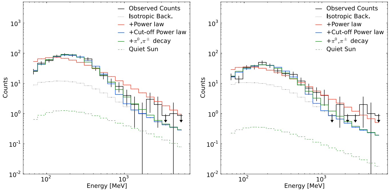
Figure 4. Comparison between observed \gamma -ray counts and predicted \gamma -ray counts for different models for the March 7 (left) and June 7 (right) solar flares. The black solid line is the histogram of the observed counts. Vertical bars are plotted using the Gehrels (1986) formula to show the expected uncertainty associated with each bin. Red, blue, and green solid lines are the expected numbers of counts for different models (background+power law, background+power law with exponential cutoff, and background+pion-decay, respectively) after likelihood maximization. The contribution of the quiet Sun is shown as a green dashed line (Abdo et al. 2011).
