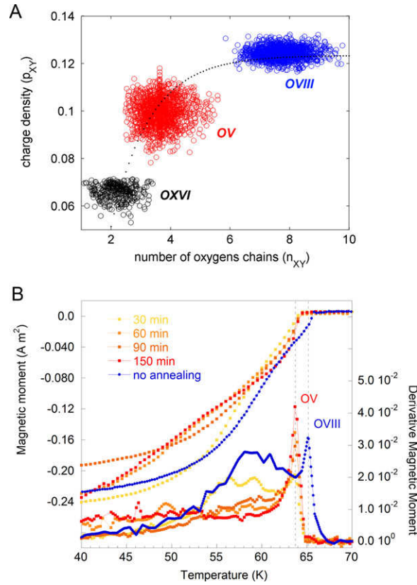
Figure 5. (a) Charge density (hole concentration p ) as a function of the number of oxygen chains, inside the OVIII, OXVI and OV puddles. The dotted curve is a fit using a model: p = 1 - \exp\{-(n - n_0)/n_0\}/\xi_n , where n_0 and \xi_n are the minimum and the maximum number of chains present in the average puddle. (b) Left scale: zero field cooling (ZFC) diamagnetic response of YBCO upon thermal cycles in an external applied field H=20 Oe. Blue filled circles: signal before any thermal annealing. Yellow–red squares: the magnetic moment upon sample annealing at 380 K with increasing dwell time of 30, 60, 90 and 150 min. Right scale: numerical derivative of the magnetic moment. Upon thermal cycling the onset of superconducting shielding decreases by about 2 K.
