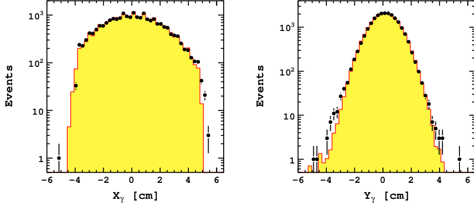
Figure 5: The reconstructed x (left) and y-positions (right) of accepted photons in the spectrometer collected in one environmental record. Dots with error bars are data and the histogram is the Monte Carlo prediction.
