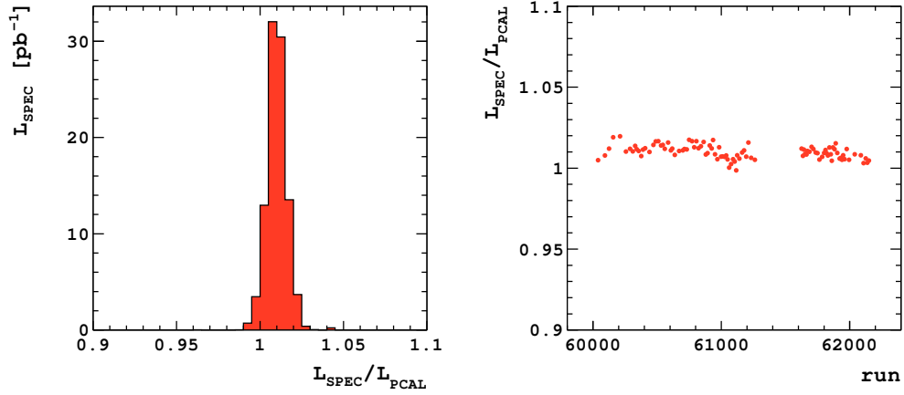
Figure 11: Left: The ratio of the luminosities measured by the spectrometer and photon calorimeter for each run, weighted with the luminosity measured using the spectrometer. Data from the 2006-2007 positron beam period are included. Right: The ratio of the luminosities measured by the spectrometer and photon calorimeter plotted against the run number. Runs are grouped to include approximately 1\text{pb}^{-1} per point.
