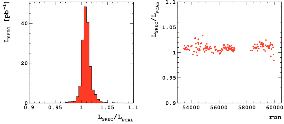
Figure 10: Left: The ratio of the luminosities measured by the spectrometer and photon calorimeter for each run, weighted with the luminosity measured using the spectrometer. Data from the 2005-2006 electron beam period are included. Right: The ratio of the luminosities measured by the spectrometer and photon calorimeter plotted against the run number. Runs are grouped to include approximately 1\text{pb}^{-1} per point.
