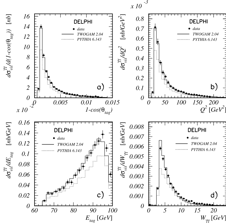
Fig. 2. Differential visible cross-sections (at LEP energies) as a function of (a) cosine of the scattered electron angle \theta_{\text{tag}} , (b) probing photon virtuality Q^2 , (c) energy of scattered electron E_{\text{tag}} , (d) visible hadronic invariant mass, for real data (points with error bars) and simulation (histograms). Visible cross sections are defined as \sigma_X = \frac{1}{L} \frac{\Delta N_{\text{sel}}}{\Delta X} where L is the integrated luminosity, N_{\text{sel}} is the number of selected events and X is the variable of interest.
