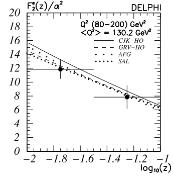
Fig. 6. LEP II data. The F_2^e measured for Q^2 \in (80, 200) \text{ GeV}^2 . For each bin the total uncertainty is plotted (the data is corrected for the absence of radiation in the theoretical prediction).
