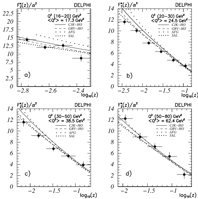
Fig. 5. LEP II data. F_2^e measured for (a) Q^2 \in (16, 20) \text{ GeV}^2 , (b) Q^2 \in (20, 30) \text{ GeV}^2 , (c) Q^2 \in (30, 50) \text{ GeV}^2 , and (d) Q^2 \in (50, 80) \text{ GeV}^2 . For each bin the total uncertainty is plotted (the data is corrected for the absence of radiation in the theoretical prediction). Note, that the AFG parametrisation is not available below \log_{10}(z) = -2.7 .
