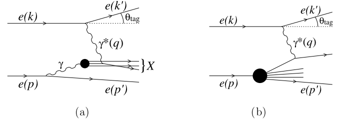
Fig. 1. Deep inelastic scattering (DIS) on a photon target (a), and on an electron target (b); p, p', k and k' denote the corresponding four-momenta and q is the four-momentum of the exchanged photon.
