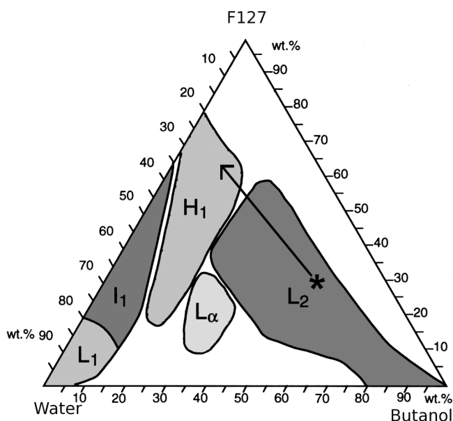
FIG. 1. Ternary phase diagram redrawn from Holmqvist et al. 38 Based on the assumption that ethanol acts as part of the oil phase together with the butanol released upon hydrolysis of titanium n -butoxide, the reaction mixture is initially in the reverse micellar phase with a composition represented by a star in the phase diagram. Rapid evaporation of solvent during the spin-coating of the sample films moves the system into the hexagonal H_1 phase of the phase diagram indicated by the arrow.
