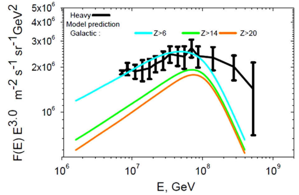
Fig. 14. Heavy component energy spectrum of Tunka 133 (Fig. 8) in comparison with the model predictions (lines are shown by the same colour as in Fig. 11). (For interpretation of the references to colour in this figure caption, the reader is referred to the web version of this paper.)
