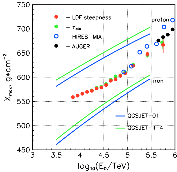
Fig. 5. Experimental X_{max} vs. primary energy.
