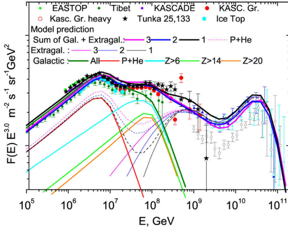
Fig. 11. All particle spectrum measured by different experiments: Tunka-133, Tunka 25 [19], KASCADE Grande [7], KASCADE [22], EASTOP [21], Tibet [20], UHE data, obtained in Hires [23], Auger [24]. Galactic cosmic rays are presented separately: dark green line (total), red line (H+He), blue line ( Z > 6 ), green one ( Z > 14 ), orange one ( Z > 20 ). Thin lines denote 3 fits of extragalactic protons, covered predictions [18]. Thick lines of the same colours represent galactic + extragalactic particles. Dashed lines denote the total light component: p+He. (For interpretation of the references to colour in this figure caption, the reader is referred to the web version of this paper.)
