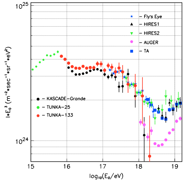
Fig. 2. Combined primary energy spectrum: comparison with some other experimental data.
