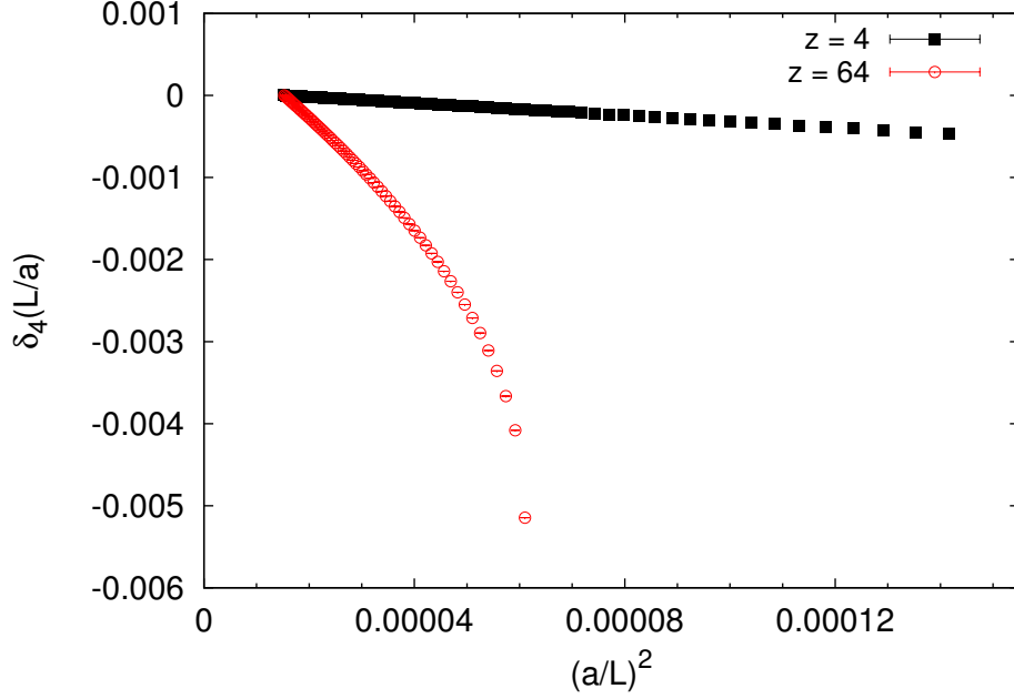
Figure 1. Tree-level results for \delta_4(L/a) defined as the difference between \Phi_4^{\text{QCD}}(1, 0.5) at a given value of L/a and \Phi_4^{\text{QCD}}(1, 0.5) at L/a = 256 , for z = 4 and z = 64 .
