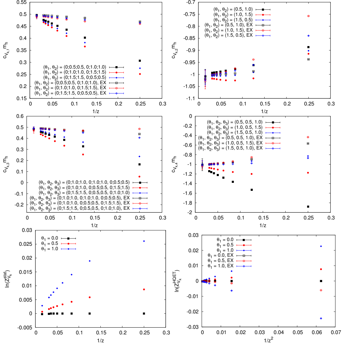
Figure 6. Tree-level continuum results for the parameters of the spatial component of the vector current.
