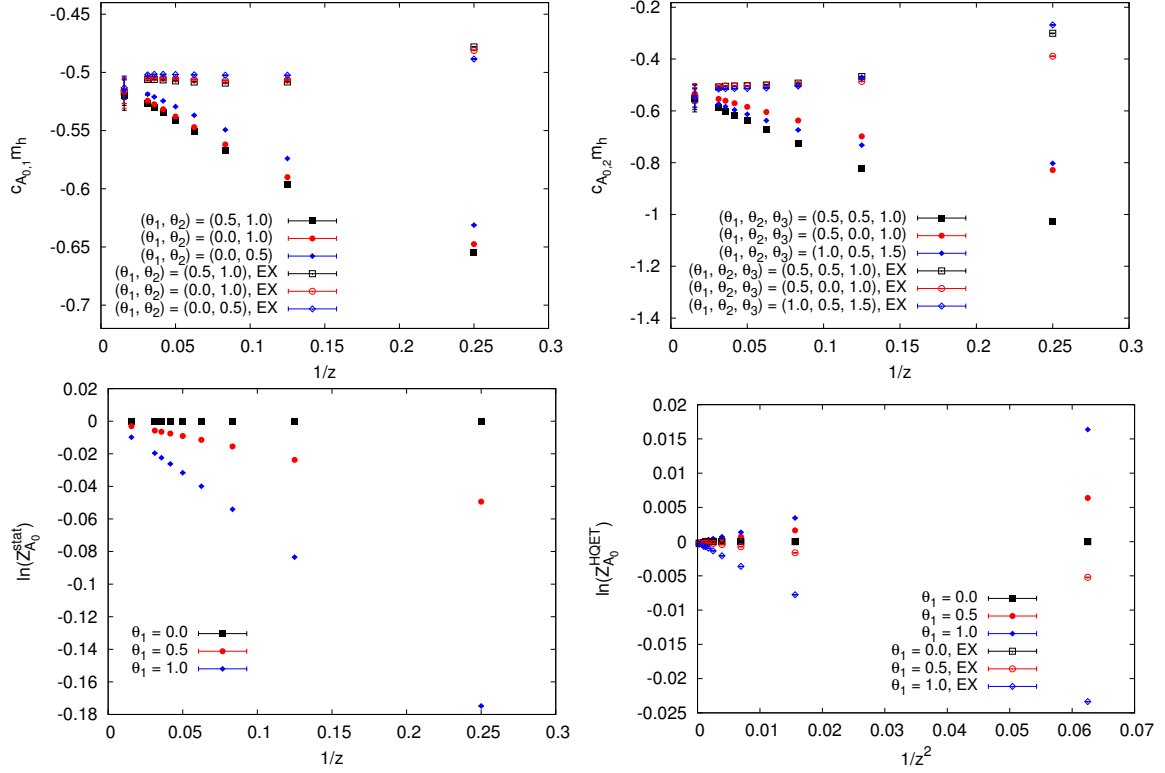
Figure 3. Tree-level continuum results for the parameters of the temporal component of the axial current.
