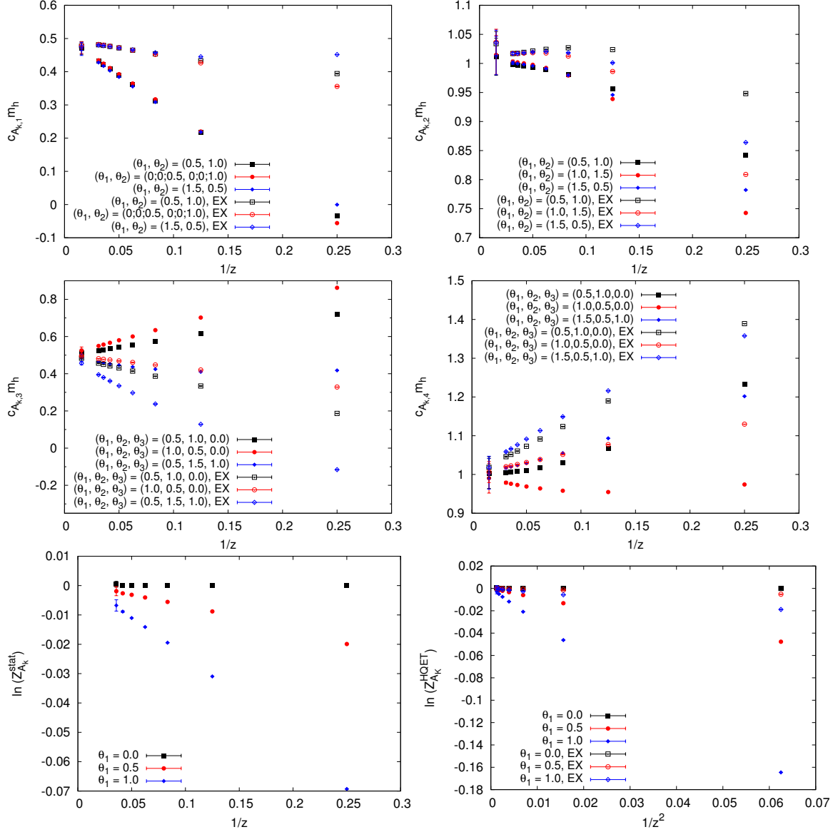
Figure 4. Tree-level continuum results for the parameters of the spatial components of the axial current.
