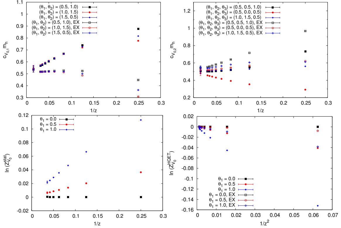
Figure 5. Tree-level continuum results for the parameters of the temporal component of the vector current.
