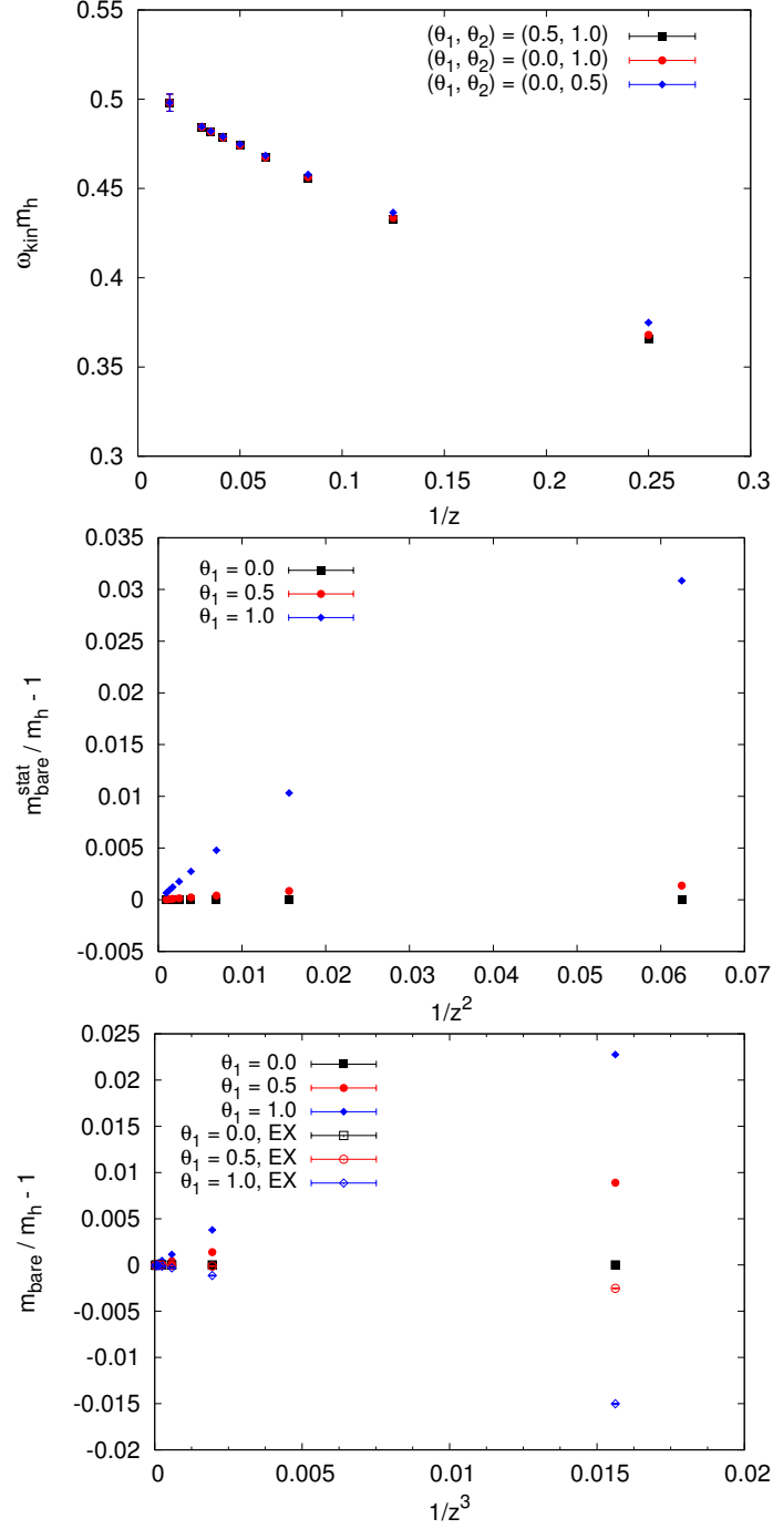
Figure 2. Tree-level continuum results for the parameters in \mathcal{L}^{\text{HQET}} .
