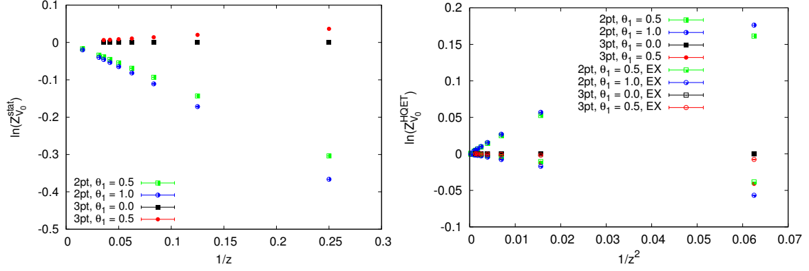
Figure 7. Comparison of tree-level continuum results for the renormalization constant of the temporal component of the vector current using either two-point correlation functions only (2pt), see eq. (B.6), or also three-point functions (3pt), as in our standard definition of \Phi_{14}^{\text{QCD}}(\vec{\theta}_1) .
