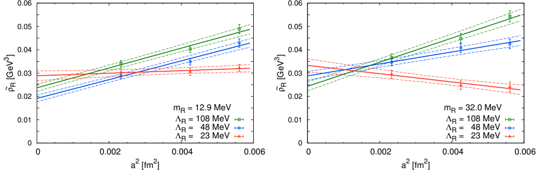
Figure 2: Effective spectral density \tilde{\rho}_R vs. the lattice spacing squared for the lightest (left hand side) and the heaviest reference quark mass m_R (right hand side), and for the lightest, an intermediate, and the heaviest cutoff \Lambda_R in both panels. In general, the data are well described by a linear fit in a^2 , which suggests that, within our statistical errors, we are in the asymptotic regime of Symanzik effective theory. As evident from the figures, there are competing (positive and negative) discretization effects, which can approximately compensate for each other in specific domains of parameter space.
