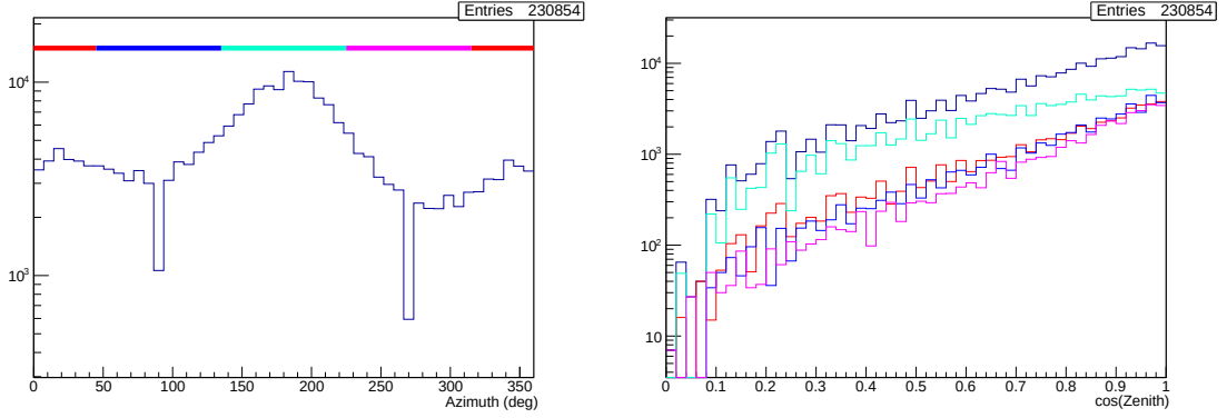
FIGURE 2. Air shower directions reconstructed from the arrival time differences in the scintillation reference detectors. The colored zenith-histograms correspond to the four different azimuthal ranges indicated by the horizontal band in the azimuth distribution.
