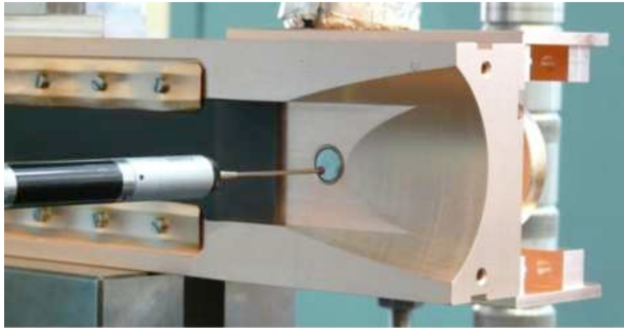
Figure 3: Zoomed view of one BPM button in the upstream jaw taper during laboratory measurements of the button position in respect to the jaw surface. [10].
