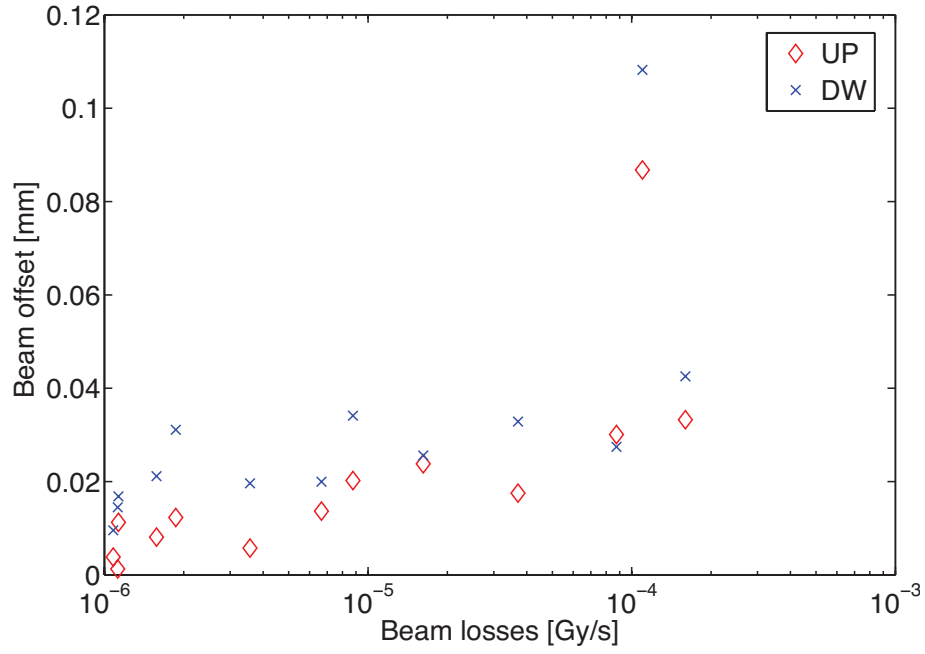
Figure 10: Beam offset measured with the upstream (red) and downstream (blue) BPMs in the mock-up collimator versus the beam loss detected by a downstream BLM. The gap of the SPS collimators was closed in twelve steps from 15 mm to 2.75 mm, resulting in a loss of 1 \times 10^{10} p.
