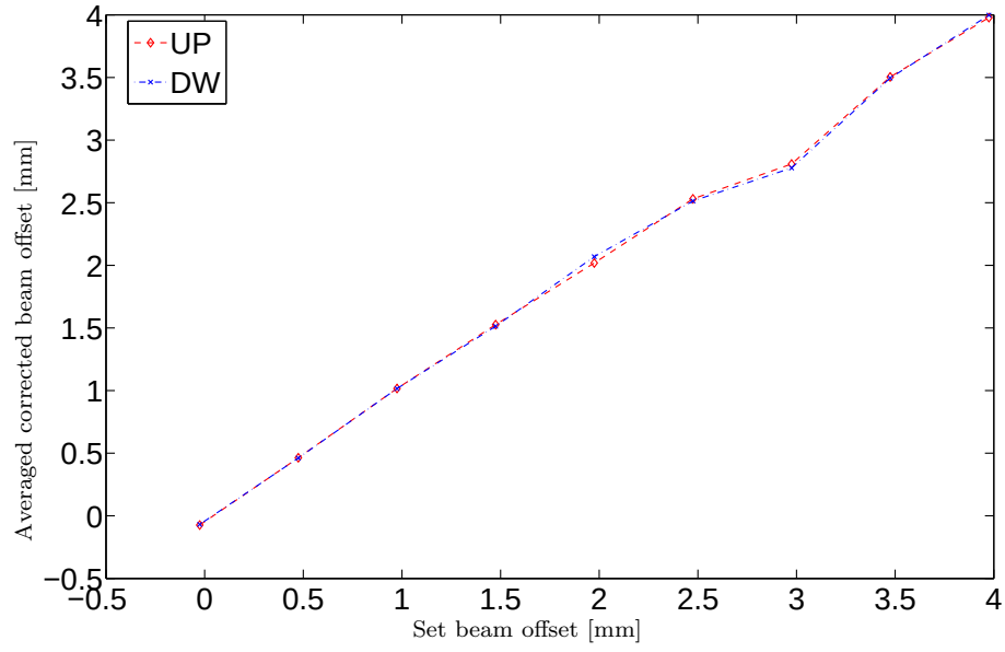
Figure 12: Measured mean beam offsets for turn-by-turn measurements (300 turns) during collimator scans at gaps of 20.35 mm for the BPM buttons at the upstream (red) and downstream (blue) end of the collimator.
