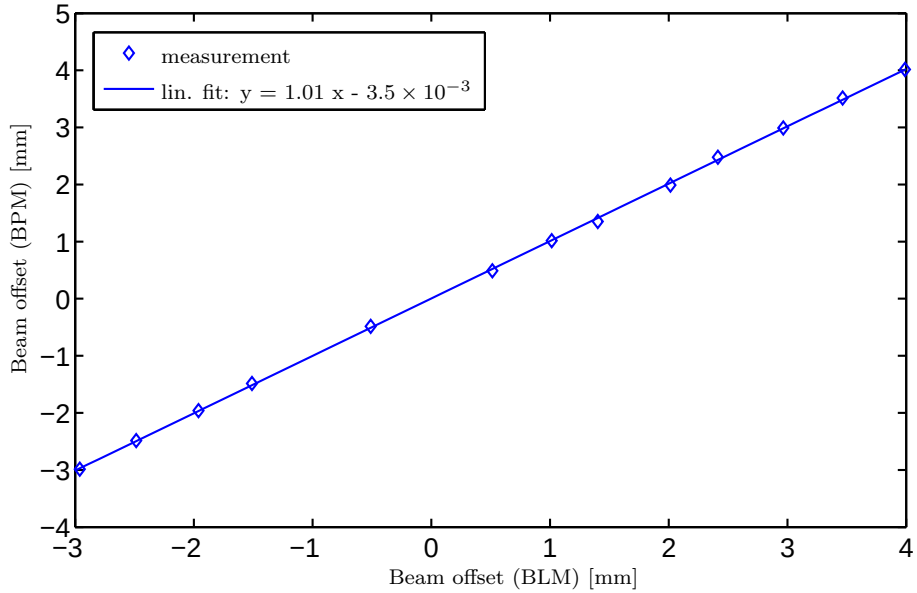
Figure 8: Correlation between beam offsets measured with the BLM-based method and the jaw-integrated BPMs (blue diamonds). The blue line shows the linear fit of the measurement data.
