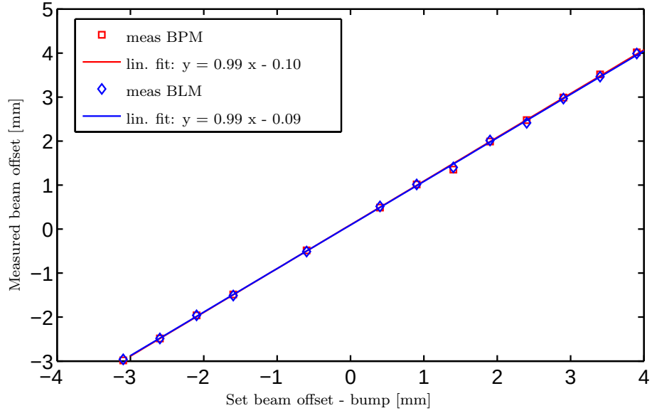
Figure 7: Correlation between measured beam centers (BPMs - red, BLM-based method - blue) and the bump settings for the orbit offset at the collimator. The error in the bump settings was estimated to about 10% of the movement increment.
