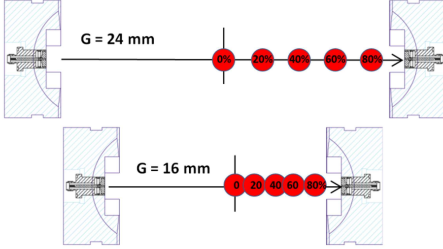
Figure 15: Collimator schematic in the transverse plane showing the simulation conditions for beam sweeps along the H-axis for different jaw gaps and beam offsets (not to scale).
