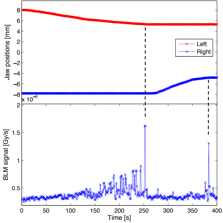
Figure 4: Jaw positions and the BLM signal during BLM-based alignment. The jaws are aligned when a spike is observed in the BLM signal, as indicated by the dashed black lines.
