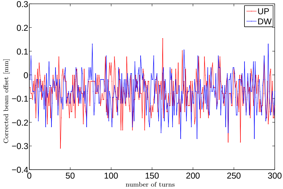
Figure 11: Corrected measured beam offsets (upstream in red, downstream in blue) versus turn number. The jaw gap was 20.35 mm and the beam offset was -0.025 mm.
