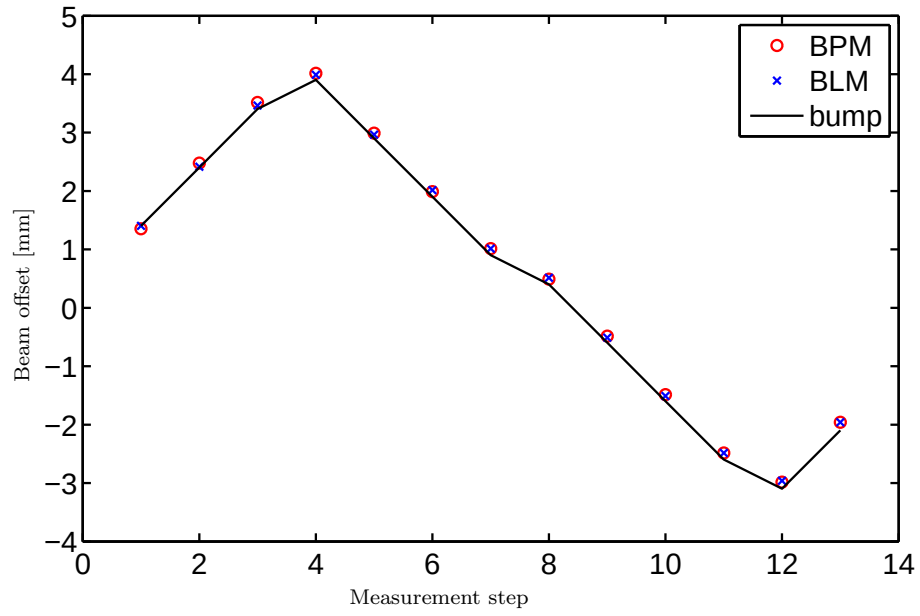
Figure 6: Comparison of the orbit offset at the collimator given by the bump (black line) and the beam offsets measured with the in-jaw BPMs (red circles) and the BLM-based alignment method (blue crosses).
