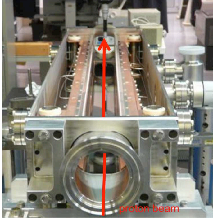
Figure 1: Photograph of the prototype collimator from one end. The moveable jaws are centred around the beam path (red arrow) and enclosed by a 1.2 m long tank.
