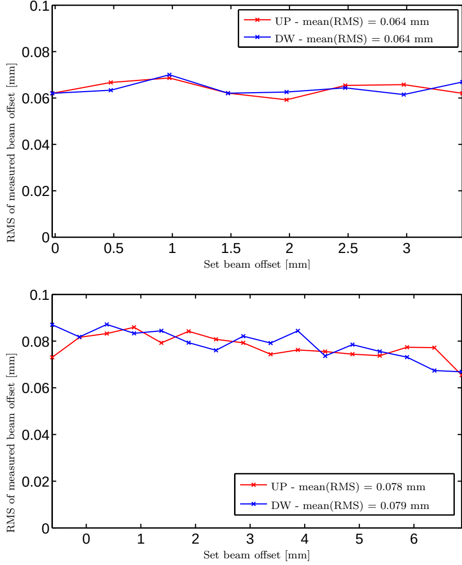
Figure 13: RMS of the beam offsets for turn-by-turn measurements (300 turns) during collimator scans at gaps of 17.35 mm (upper) and 24.75 mm (lower) for the BPM buttons at the upstream (red) and downstream (blue) end of the collimator.
