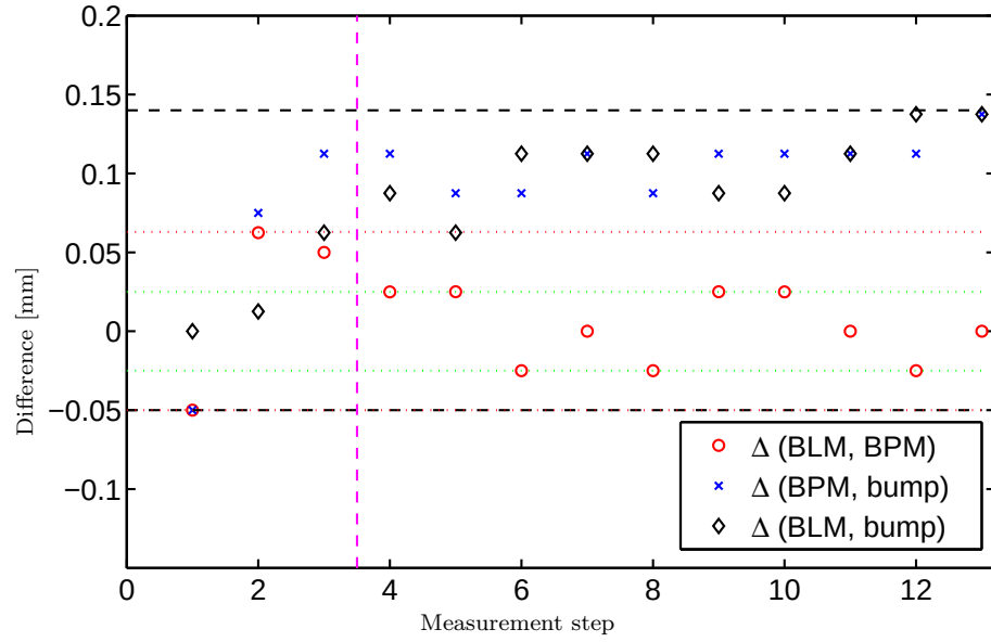
Figure 9: Differences between bump settings and beam offsets measured with the in-jaw BPMs (blue crosses) and the BLM-based method (black diamonds) respectively. The differences of measured beam offsets between the BPM and BLM-based method are shown as red circles. The vertical magenta dashed line indicates the end of an additional external orbit drift during the first 30 mins of the measurement. The horizontal dotted green lines indicate the maximum deviation between the beam offsets measured with the BPMs and the BLM-based methods, if the data during the orbit drift are not included.
