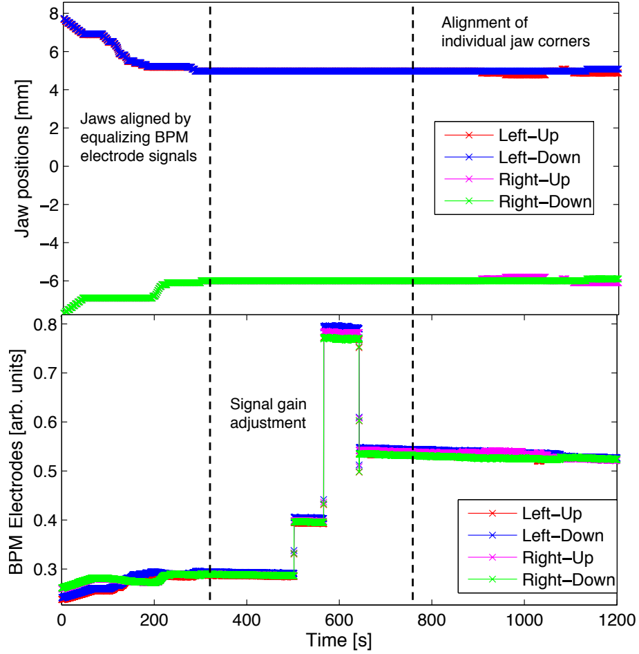
Figure 5: Jaw positions and BPM electrode signals during BPM-based alignment. The electrode signal gain was changed to reduce the non-linearities in the electronics.
