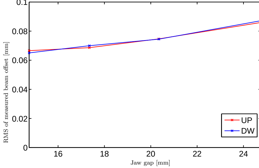
Figure 14: Measured maximum RMS of the beam offset versus collimator gap for the BPM buttons at the upstream (red) and downstream (blue) end of the collimator.
