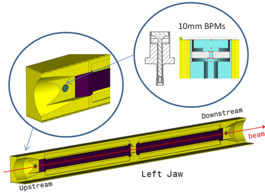
Figure 2: A model of a single jaw of the prototype collimator with embedded BPM pick-ups at both ends.
