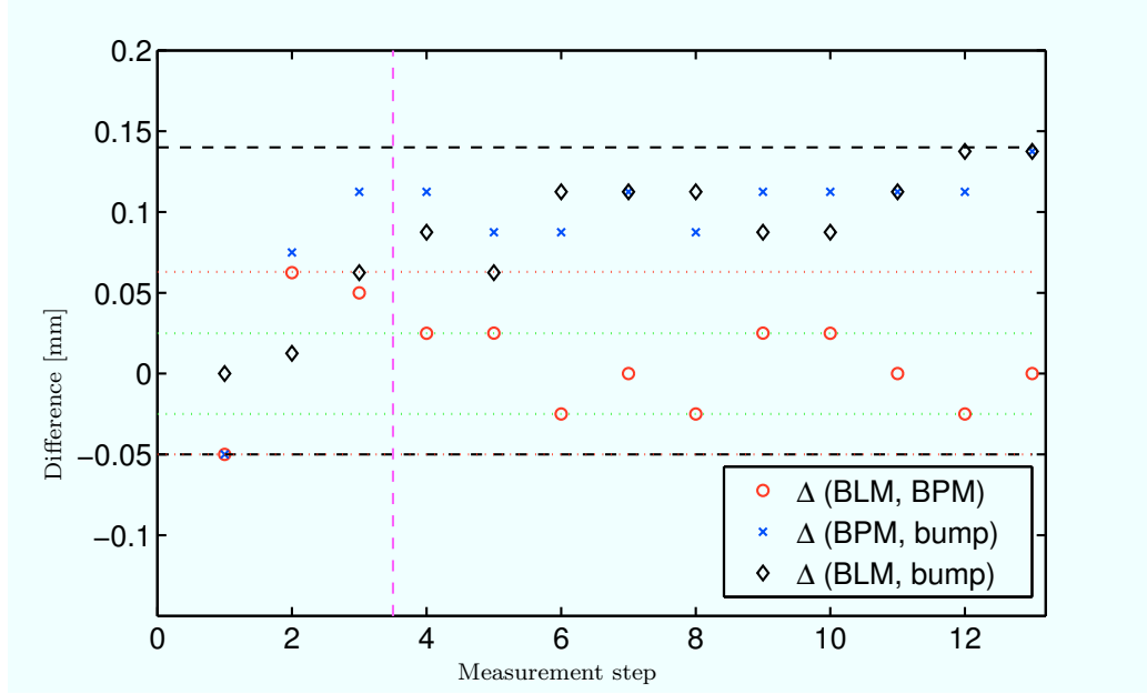
Figure 9: Differences between bump settings and beam offsets measured with the in-jaw BPMs (blue crosses) and the BLM-based method (black diamonds) respectively. The differences of measured beam offsets between the BPM and BLM-based method are shown as red circles. The vertical magenta dashed line indicates the end of an additional external orbit drift during the first 30 mins of the measurement. The horizontal dotted green lines indicate the maximum deviation between the beam offsets measured with the BPMs and the BLM-based methods, if the data during the orbit drift are not included.
