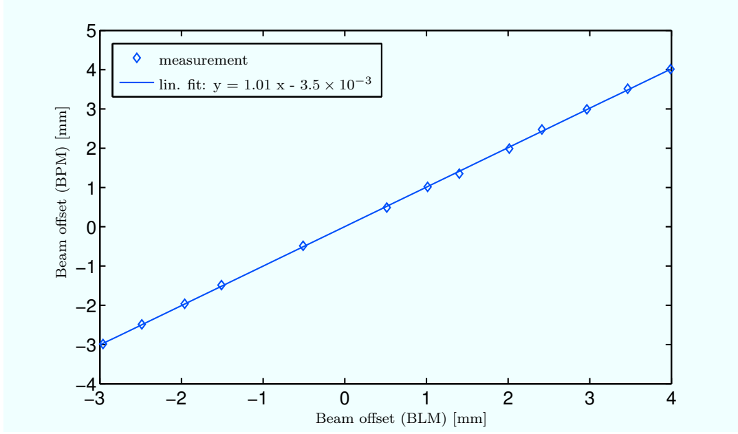
Figure 8: Correlation between beam offsets measured with the BLM-based method and the jaw-integrated BPMs (blue diamonds). The blue line shows the linear fit of the measurement data.
