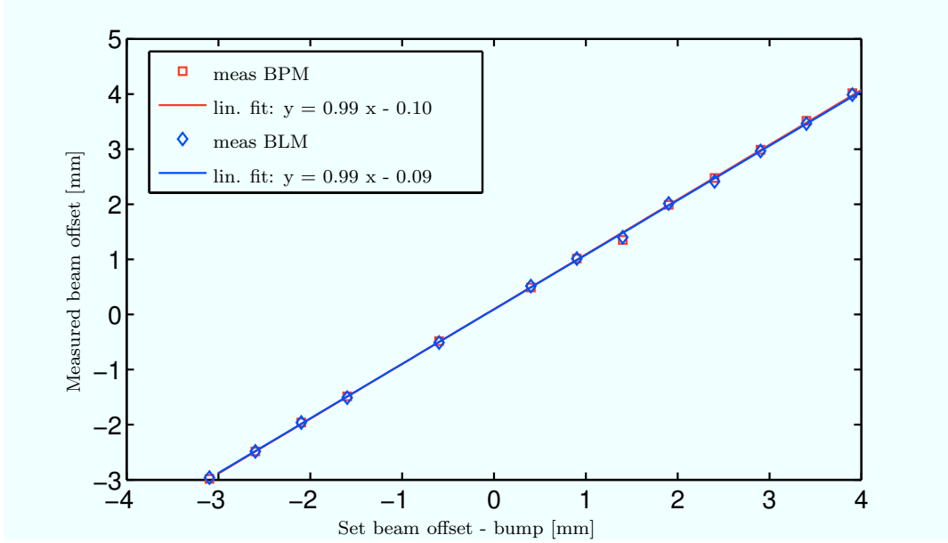
Figure 7: Correlation between measured beam centers (BPMs - red, BLM-based method - blue) and the bump settings for the orbit offset at the collimator. The error in the bump settings was estimated to about 10% of the movement increment.
