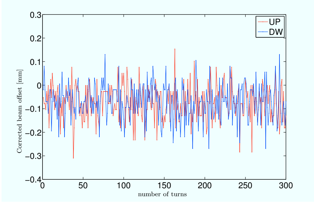
Figure 11: Corrected measured beam offsets (upstream in red, downstream in blue) versus turn number. The jaw gap was 20.35 mm and the beam offset was -0.025 mm.
