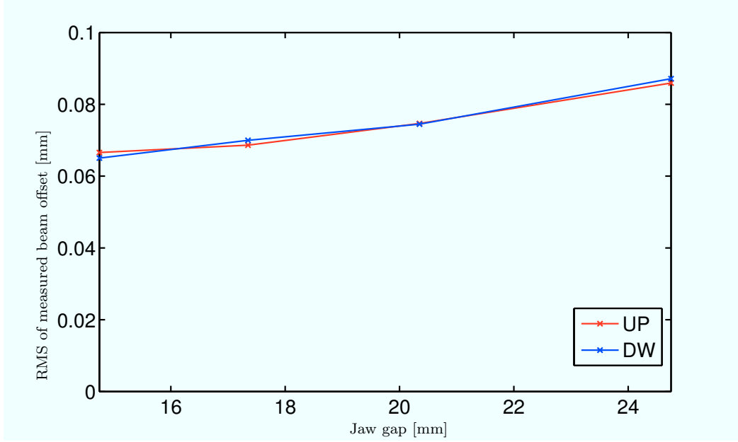
Figure 14: Measured maximum RMS of the beam offset versus collimator gap for the BPM buttons at the upstream (red) and downstream (blue) end of the collimator.
