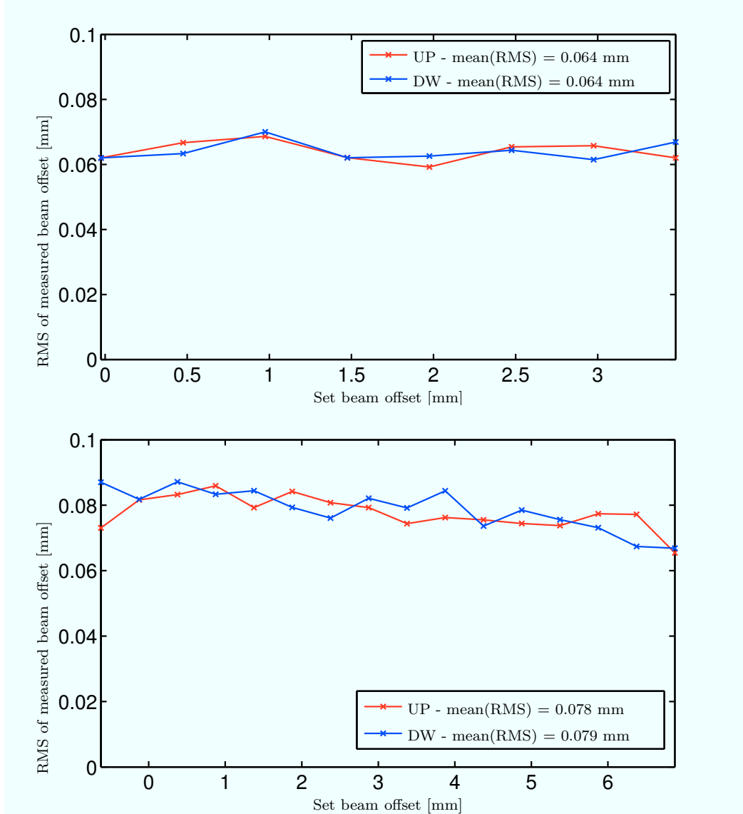
Figure 13: RMS of the beam offsets for turn-by-turn measurements (300 turns) during collimator scans at gaps of 17.35 mm (upper) and 24.75 mm (lower) for the BPM buttons at the upstream (red) and downstream (blue) end of the collimator.
