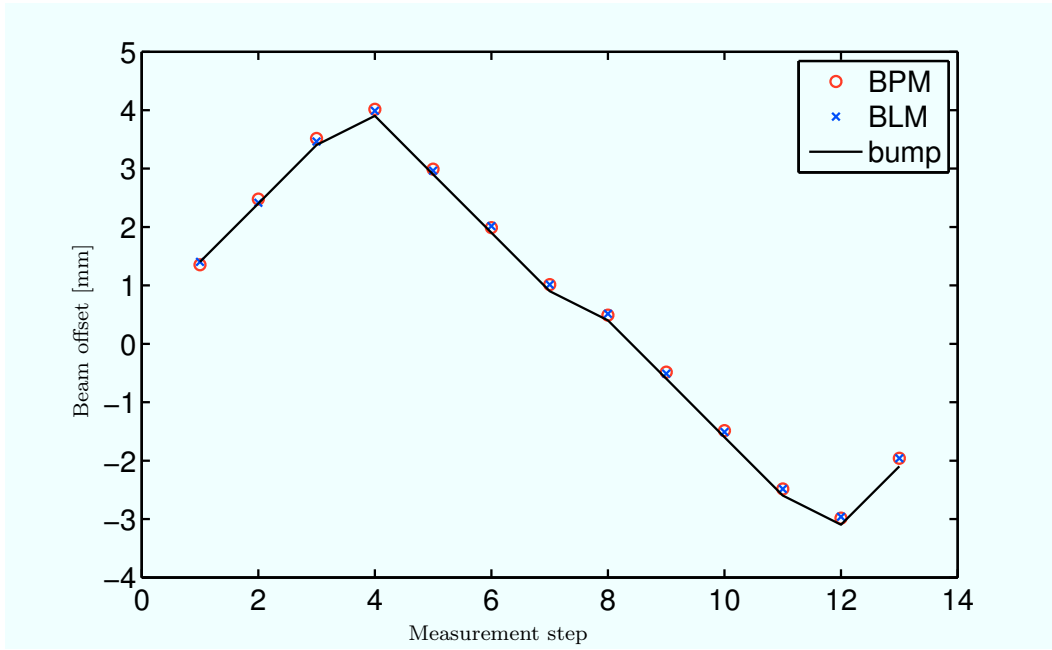
Figure 6: Comparison of the orbit offset at the collimator given by the bump (black line) and the beam offsets measured with the in-jaw BPMs (red circles) and the BLM-based alignment method (blue crosses).
