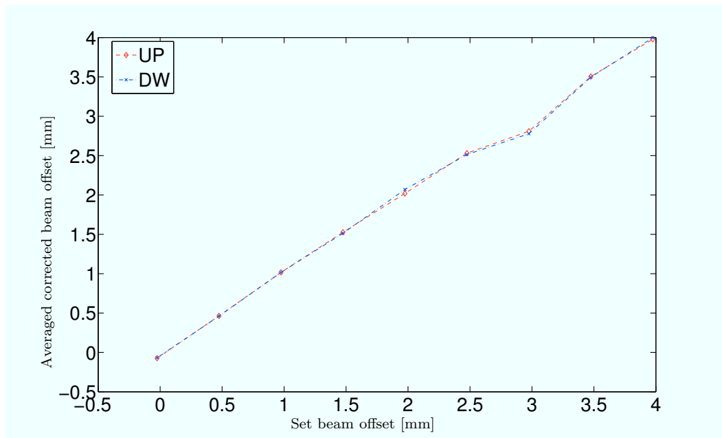
Figure 12: Measured mean beam offsets for turn-by-turn measurements (300 turns) during collimator scans at gaps of 20.35 mm for the BPM buttons at the upstream (red) and downstream (blue) end of the collimator.
