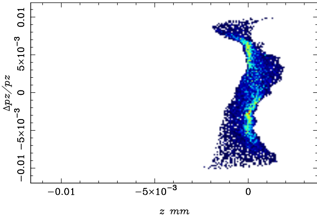
Figure 6: Longitudinal phase space after correction with a 3 rd harmonic rf cavity; the scale of the abscissa corresponds to Fig. 4. The initial distribution has a parabolic line charge density; the rms bunch length is 0.6 μm (2 fs).
