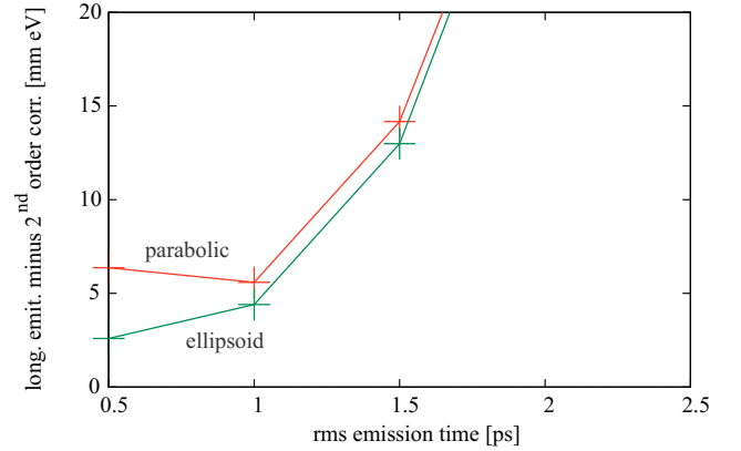
Figure 10: 2^{nd} order corrected longitudinal emittance as function of the laser pulse length behind the buncher cavity ( z = 1.6 m).
