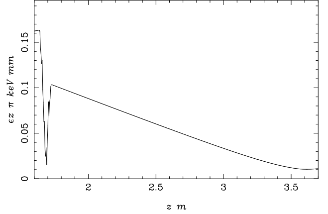
Figure 7: Development of the longitudinal emittance in the 3 rd harmonic cavity ( z = 1.65 m) and downstream up to the longitudinal focus at z = 3.6 m
