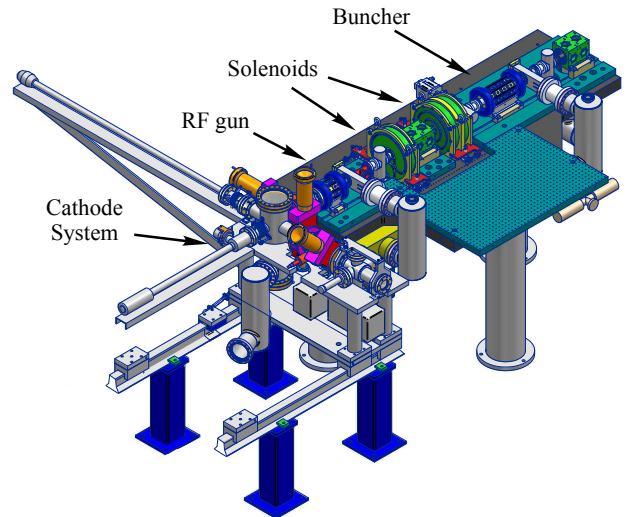
Figure 1: The first section of the REGAE facility.
