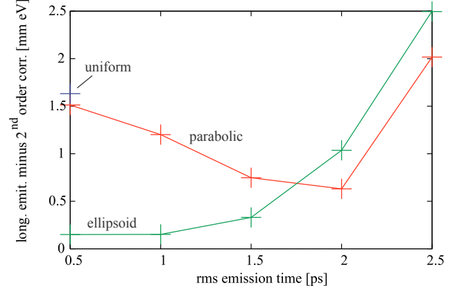
Figure 9: 2^{nd} order corrected longitudinal emittance as function of the laser pulse length just after emission from the cathode ( z = 9 \cdot 10^{-5} m). Only one data point is shown for the uniform distribution.
