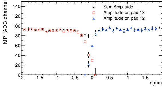
Figure 32: The MPV of the signal amplitude as a function of the hit position on the border between two adjacent pads. The star points represent the sum signal of the two neighboring pads for each strip.
