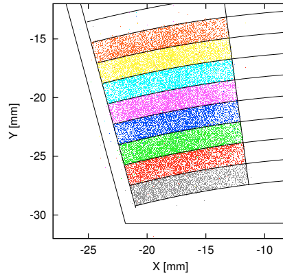
Figure 20: Reconstructed position of impact point on the sensor with color assignment corresponding to the pad with hits above threshold, registered in the LumiCal.
