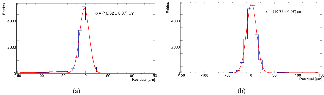
Figure 14: (a) Residual distribution on the X direction. (b) Residual distribution on the Y direction.
