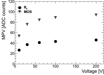
Figure 27: The signal amplitude as a function of the applied bias voltage measured using FE ASICs with R_f and MOS feedback.
