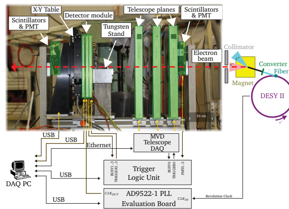
Figure 13: Scheme of the beam setup from the 2011 test period.
