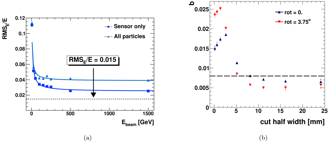
Figure 5: (a) The expected LumiCal relative resolution \frac{RMS_E}{E} as a function of the electron energy E , for showers uniformly distributed over the fiducial volume of LumiCal without and with a requirement that the shower be started within the sensors area. (b) The expected value of the resolution constant term, b , as a function of the minimal required distance of the reconstructed shower position from the middle of the tile gap.
