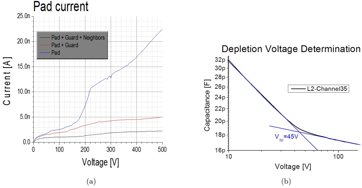
Figure 17: (a) The current I as a function of the voltage V for various measurement setups. (b) The capacitance versus voltage of a selected sensor.
