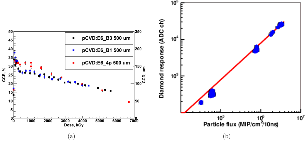
Figure 20: (a) The CCE as a function of the absorbed dose for the pCVD diamond sensors. (b) The response of polycrystalline diamond sensors as a function of the particle flux in units of the number of particles per 10 ns.
