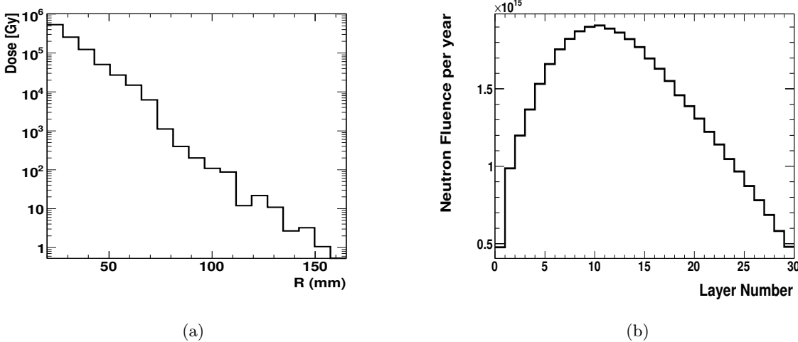
Figure 11: (a) The dose in BeamCal sensors per year as a function of the radial distance from the beam. (b) The fluence of neutrons per year inside the sensors of BeamCal as a function of the sensor layer number using the cascade model of Bertini. A centre of mass energy of 0.5 TeV is assumed
