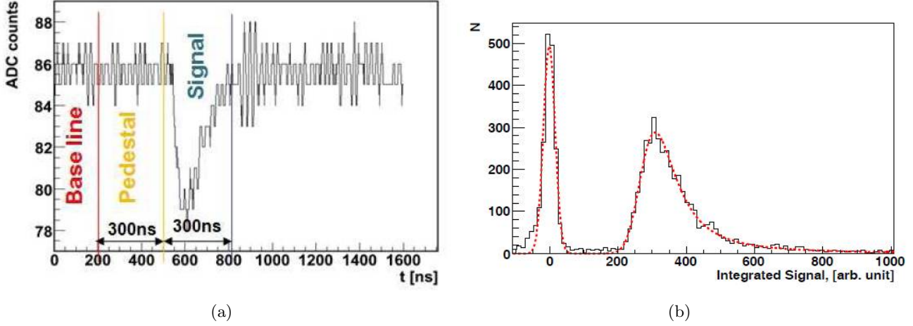
Figure 34: (a) A digitized signal of one channel recorded with a 500 Ms/s ADC. (b) The spectrum of triggered events. The signal is integrated over the wavefront in (a).
