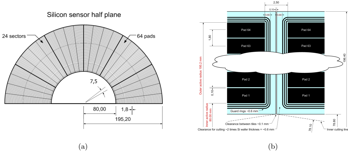
Figure 16: (a) A half plane of one of the LumiCal sensors. (b) Details of the gap-structure of the LumiCal silicon sensor.
