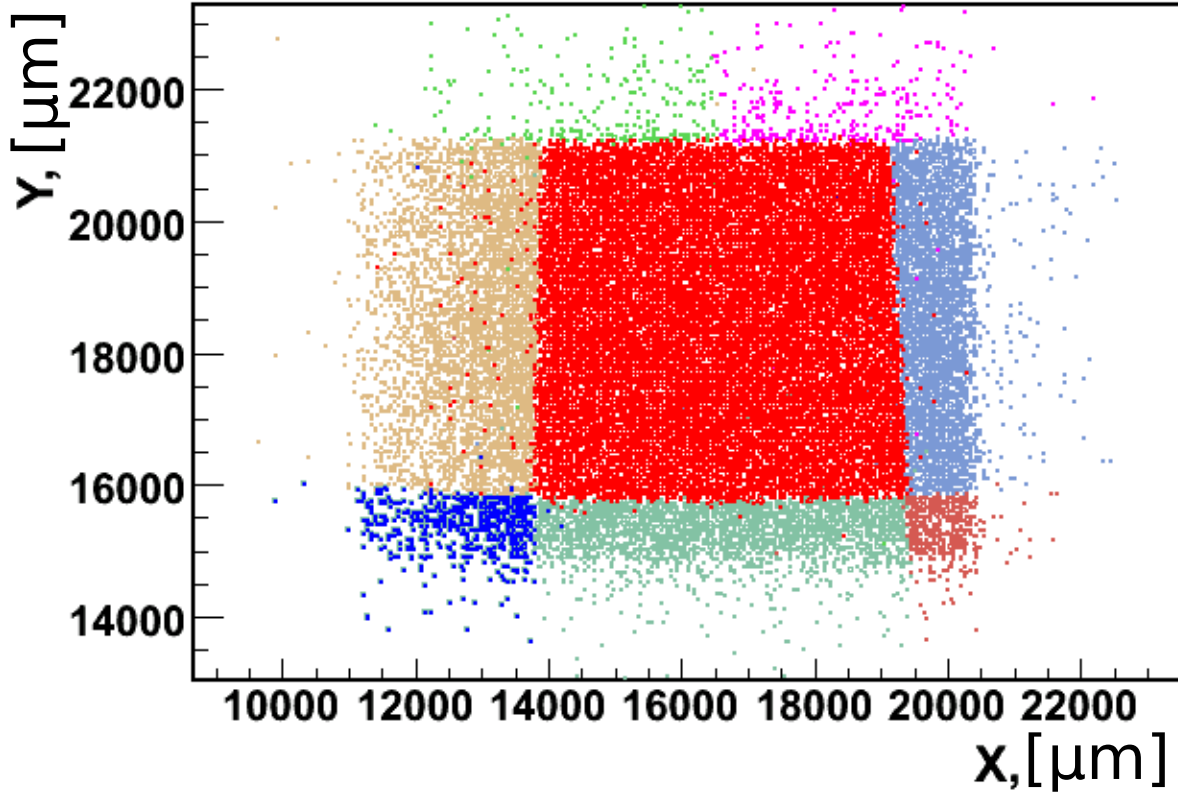
Figure 35: Pads struture of the GaAs sensor reonstruted from telescope data.
