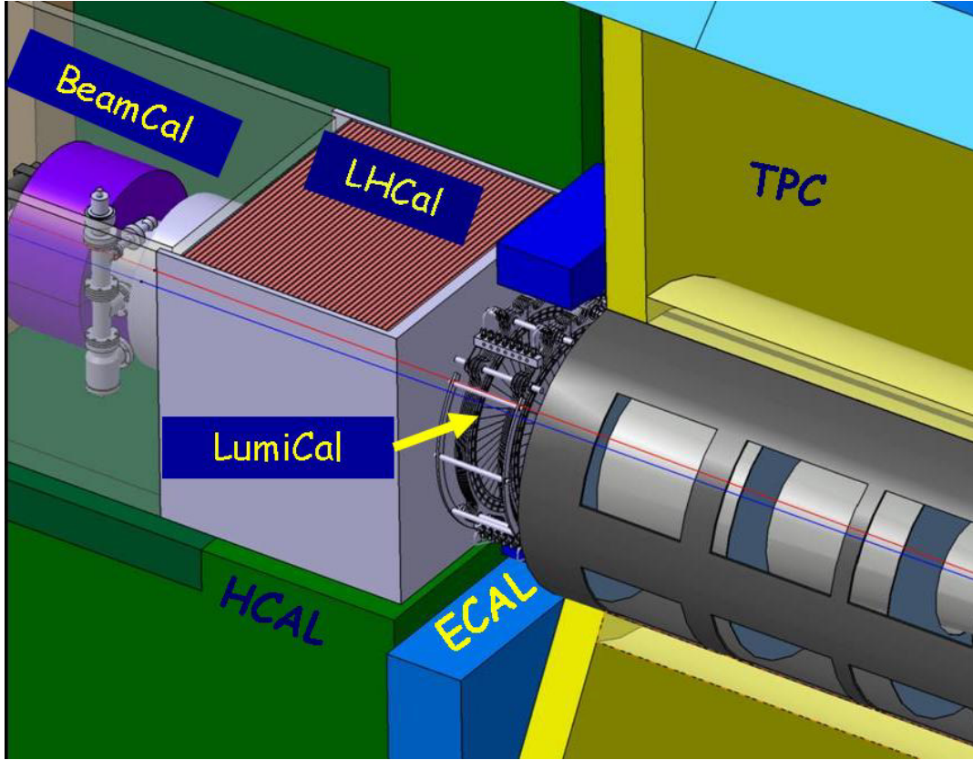
Figure 1: The very forward region of the ILD detector. LumiCal, BeamCal and LHCaI are carried by the support tube for the final focusing quadrupole and the beam-pipe. LHCaI extends the coverage of the hadron calorimeter to the polar angle range of LumiCal. TPC denotes the central track chamber, ECAL the electromagnetic and HCAL the hadron calorimeter.
