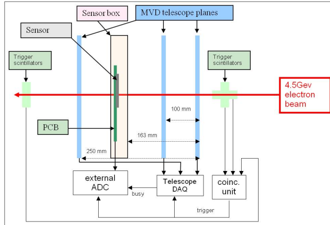
Figure 33: Scheme of the beam tests set-up.
