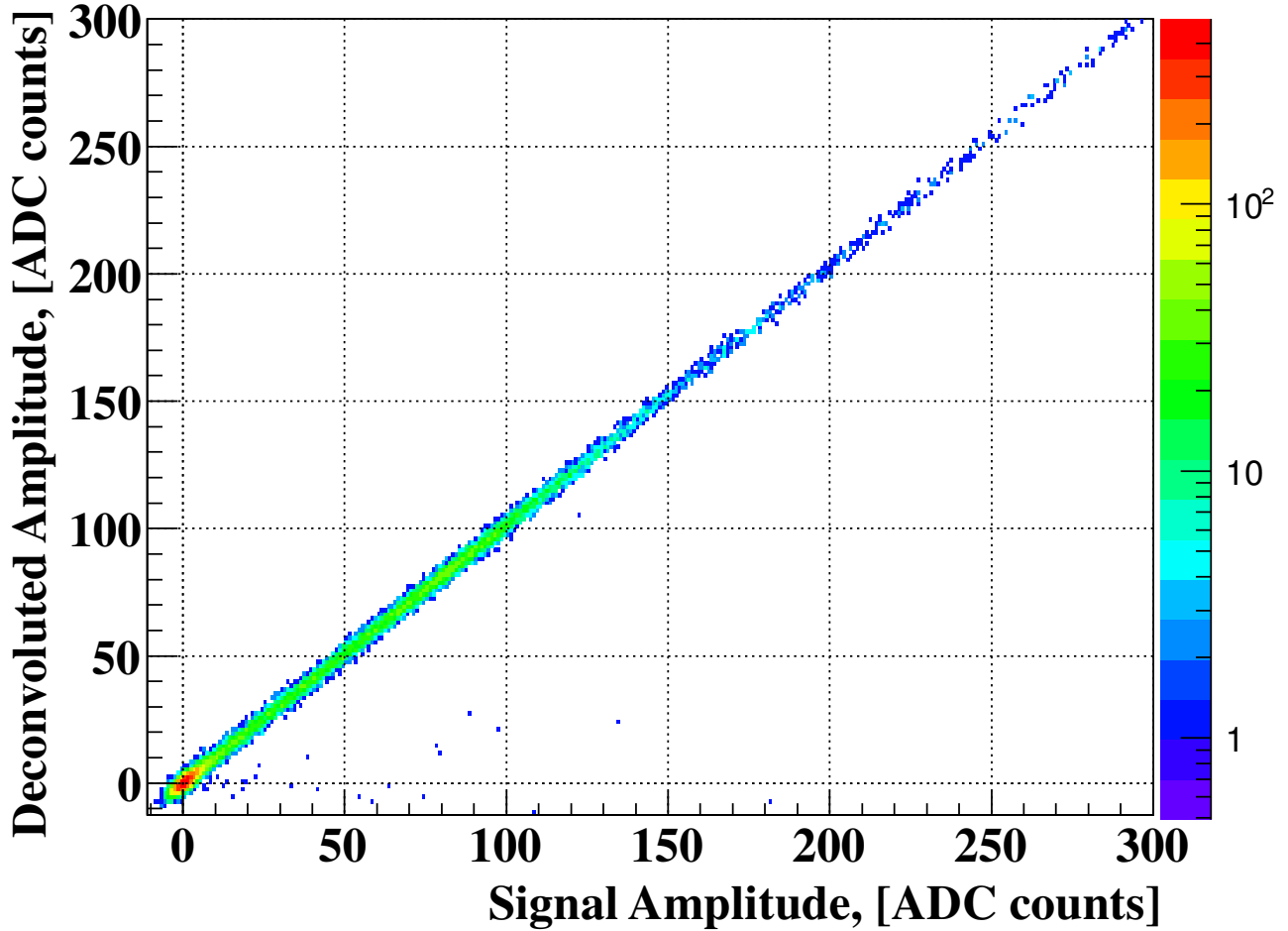
Figure 40: The deconvoluted amplitude as a function of the signal amplitude for the synchronous read out mode.
