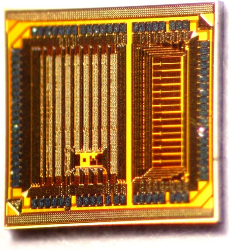
Figure 29: Photograph of ADC prototype in CMOS 130 nm technology.
