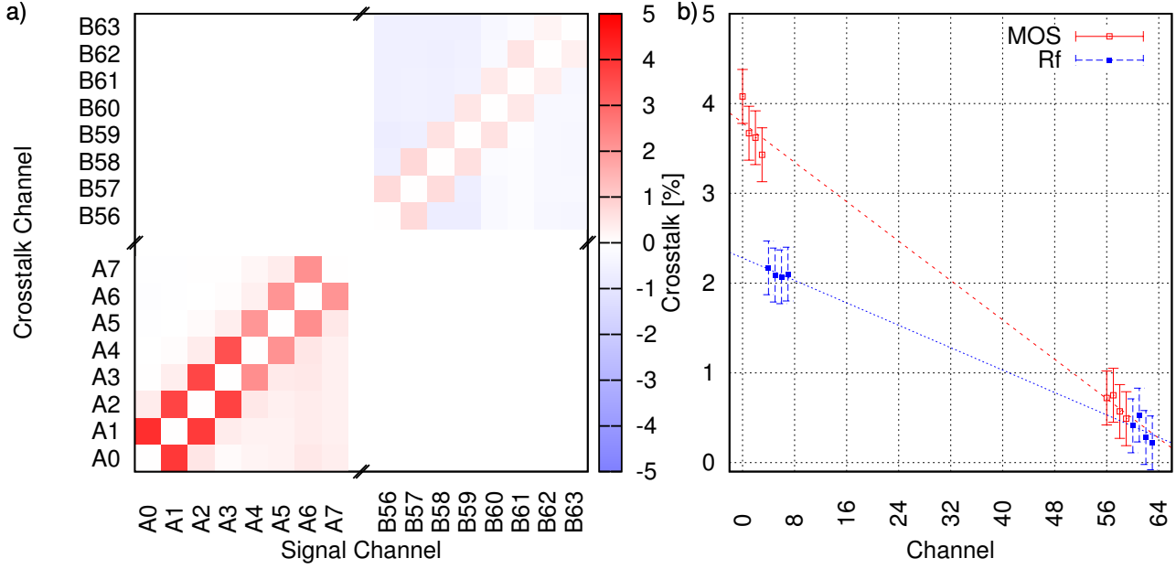
Figure 46: a) Measured crosstalk coefficients for groups of eight pads. b) Measured crosstalk coefficients to the closest neighbor as a function of pad number.
