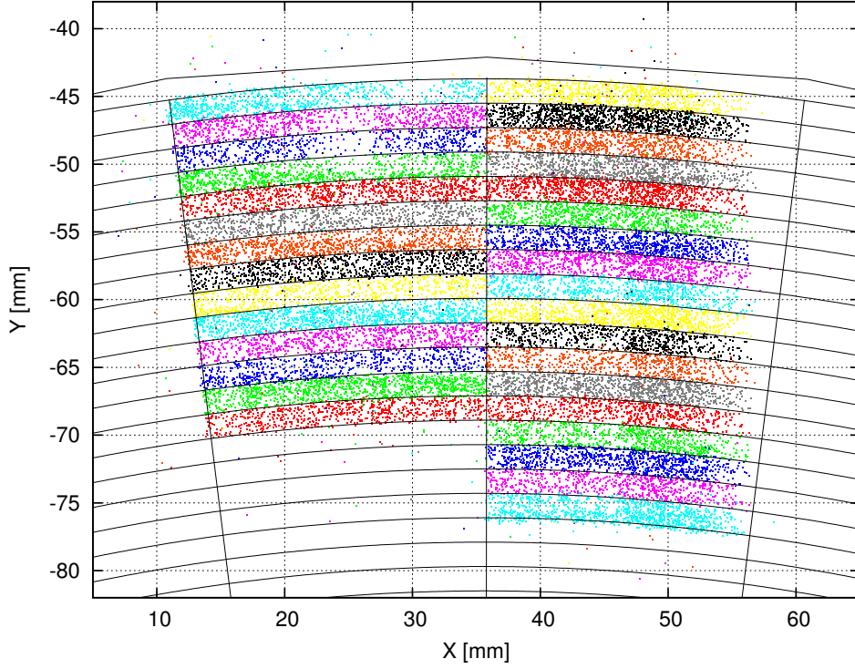
Figure 47: Reconstructed position of impact point on sensor with color assigned correspond to the pad with hit above threshold registered in the LumiCal at the 2011 beam test.
