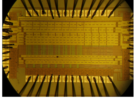
Figure 26: Micrograph of front-end ASIC.
