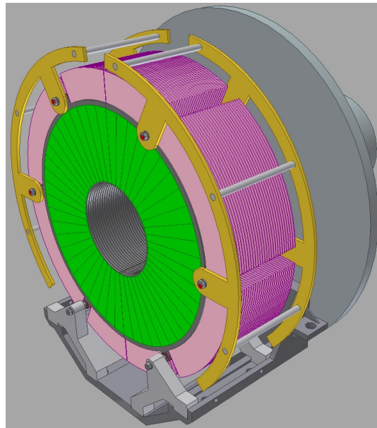
Figure 15: The mechanical structure of LumiCal. Tungsten disks are precisely positioned using 4 bolts which are stabilised by additional steel rings on both sides of the cylinder.
