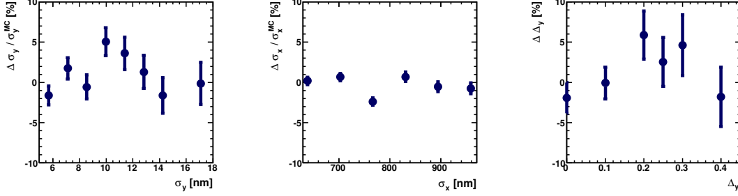
Figure 13: The relative deviations of the vertical, \sigma_y , and horizontal, \sigma_x , beam sizes, and the ratio of vertical displacement to the vertical beam size, \Delta_y , averaged over 50 bunch crossings which are measured by the pair monitor.
